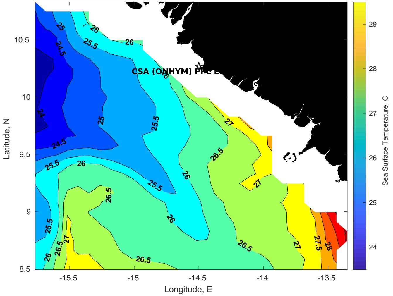
SST for CSA (ONHYM) PPL EBS - Guinea at 30-Mar-2025 00:00:00
