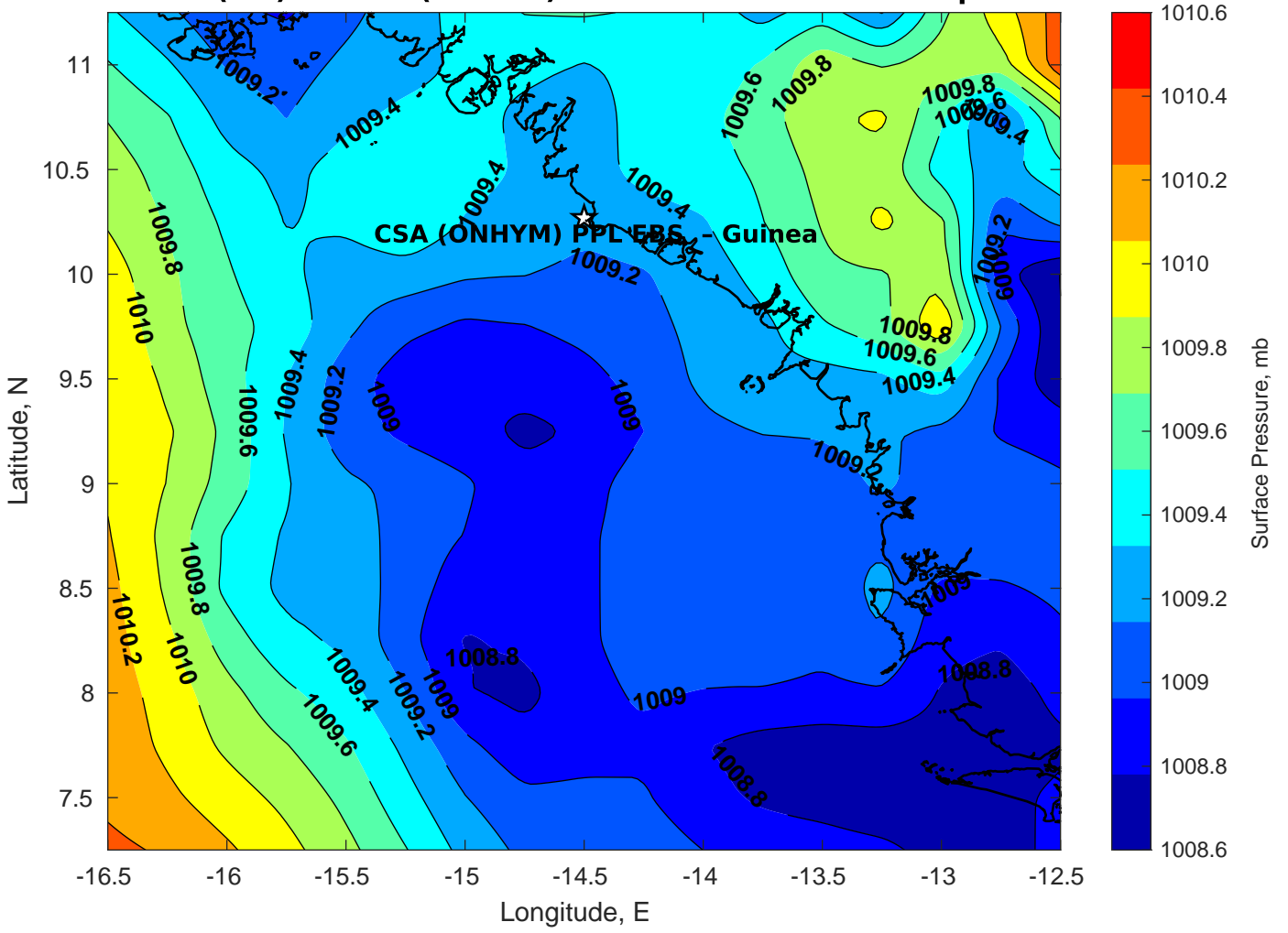
Surface Pressure (mb) for CSA (ONHYM) PPL EBS - Guinea at 02-Apr-2025 00:00:00
