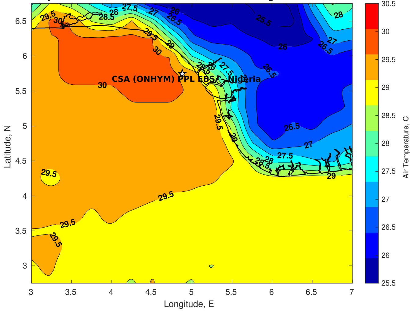
Air Temperature (C) for CSA (ONHYM) PPL EBS - Nigeria at 31-Mar-2025
