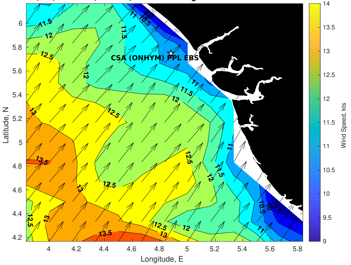
Winds (kts) for CSA (ONHYM) PPL EBS - Nigeria at 31-Mar-2025 09:00:00
