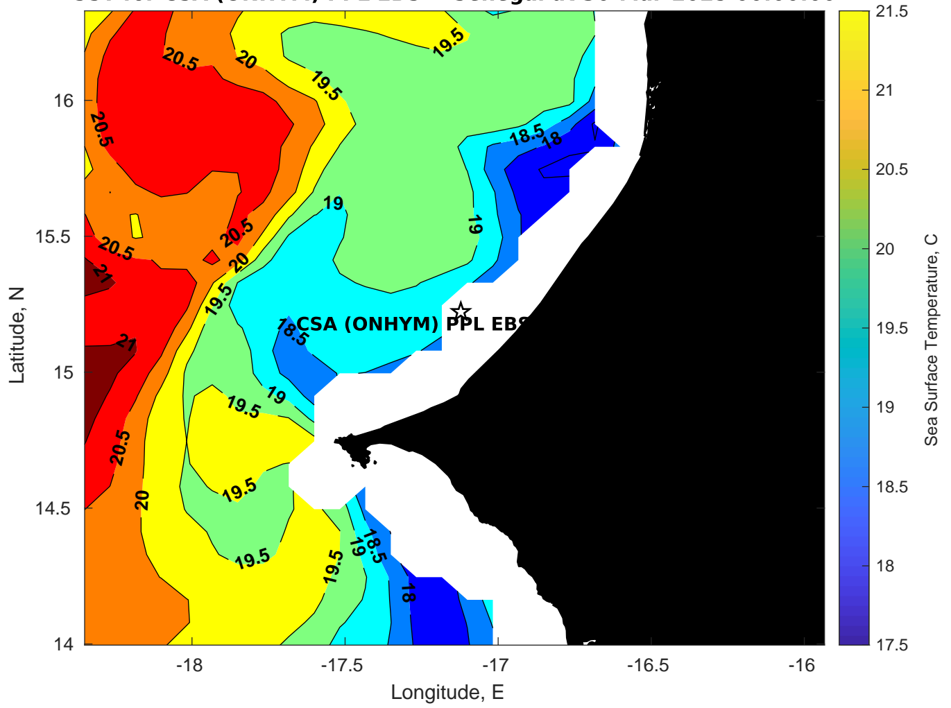
SST for CSA (ONHYM) PPL EBS - Senegal at 30-Mar-2025 00:00:00
