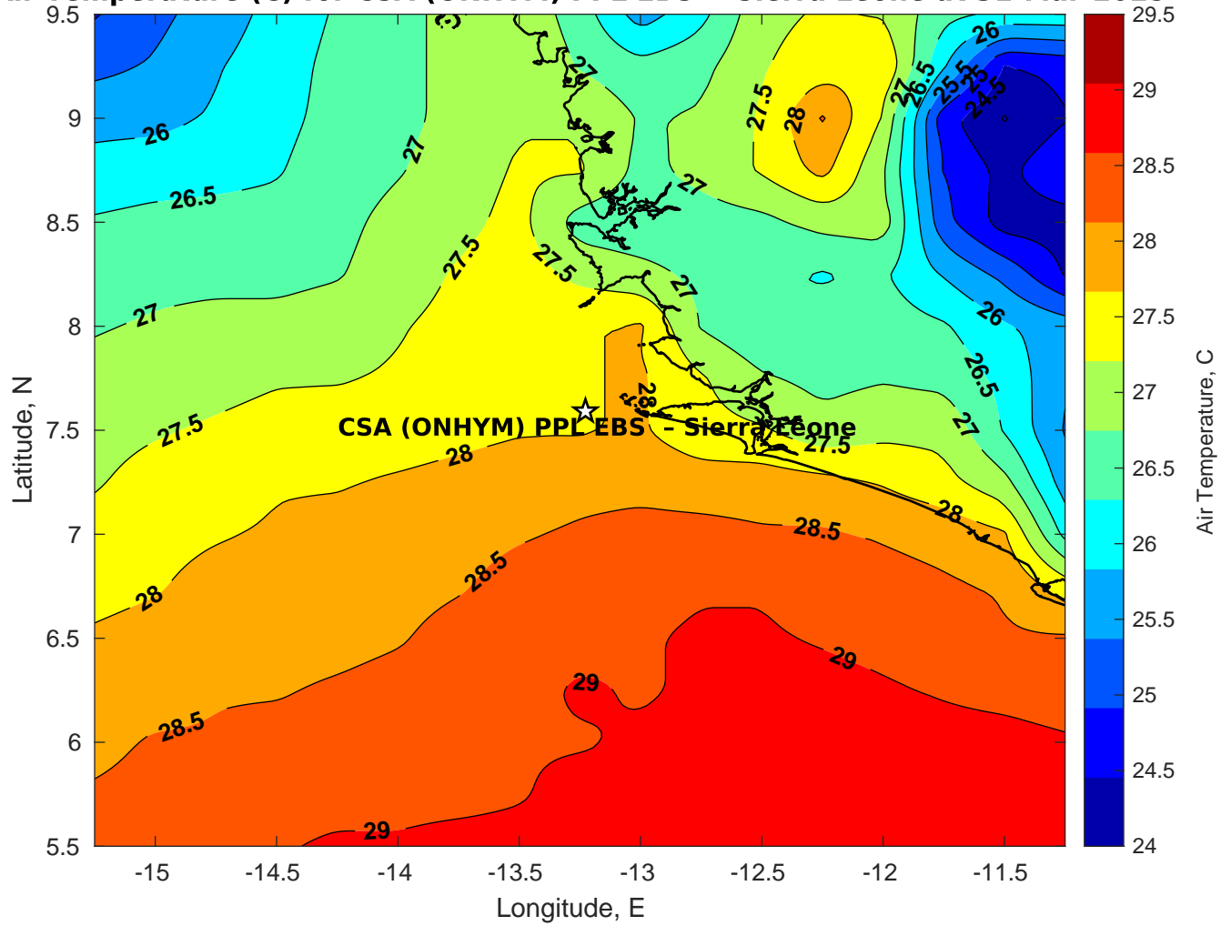
Air Temperature (C) for CSA (ONHYM) PPL EBS - Sierra Leone at 31-Mar-2025
