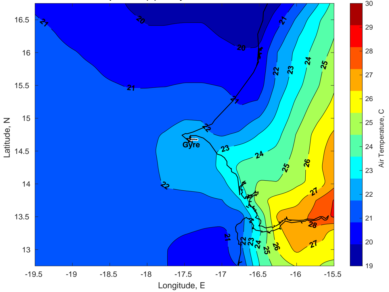
Air Temperature (C) for Gyre at 31-Mar-2025
