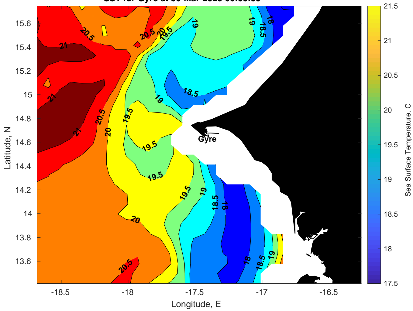
SST for Gyre at 30-Mar-2025 00:00:00
