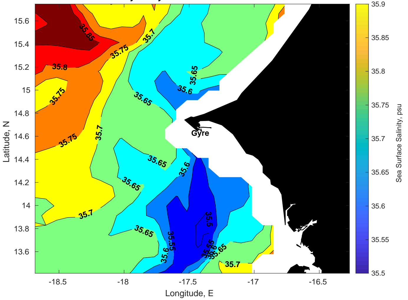
Surface Salinity for Gyre at 30-Mar-2025 00:00:00
