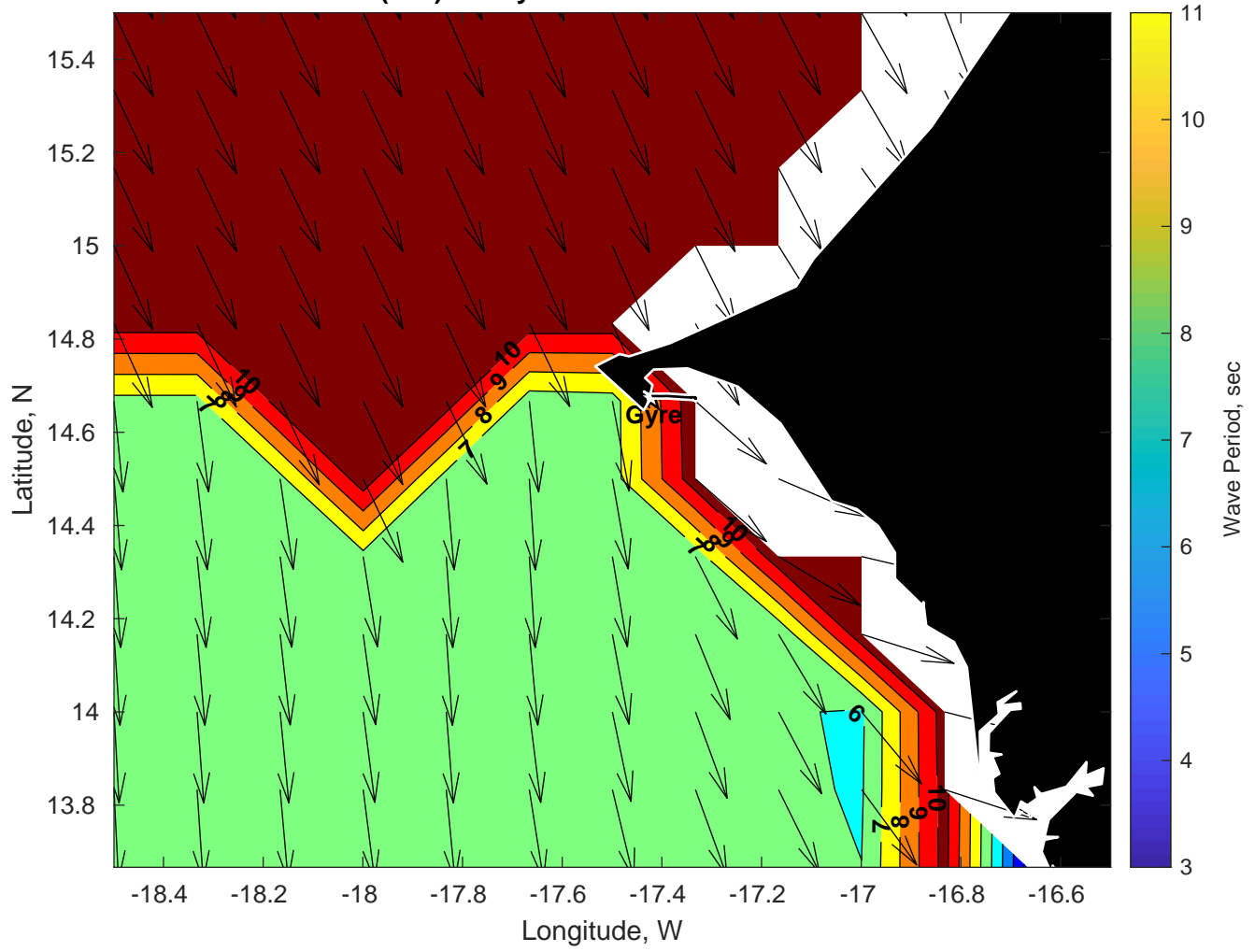
Wave Period (sec) for Gyre at 31-Mar-2025 09:00:00
