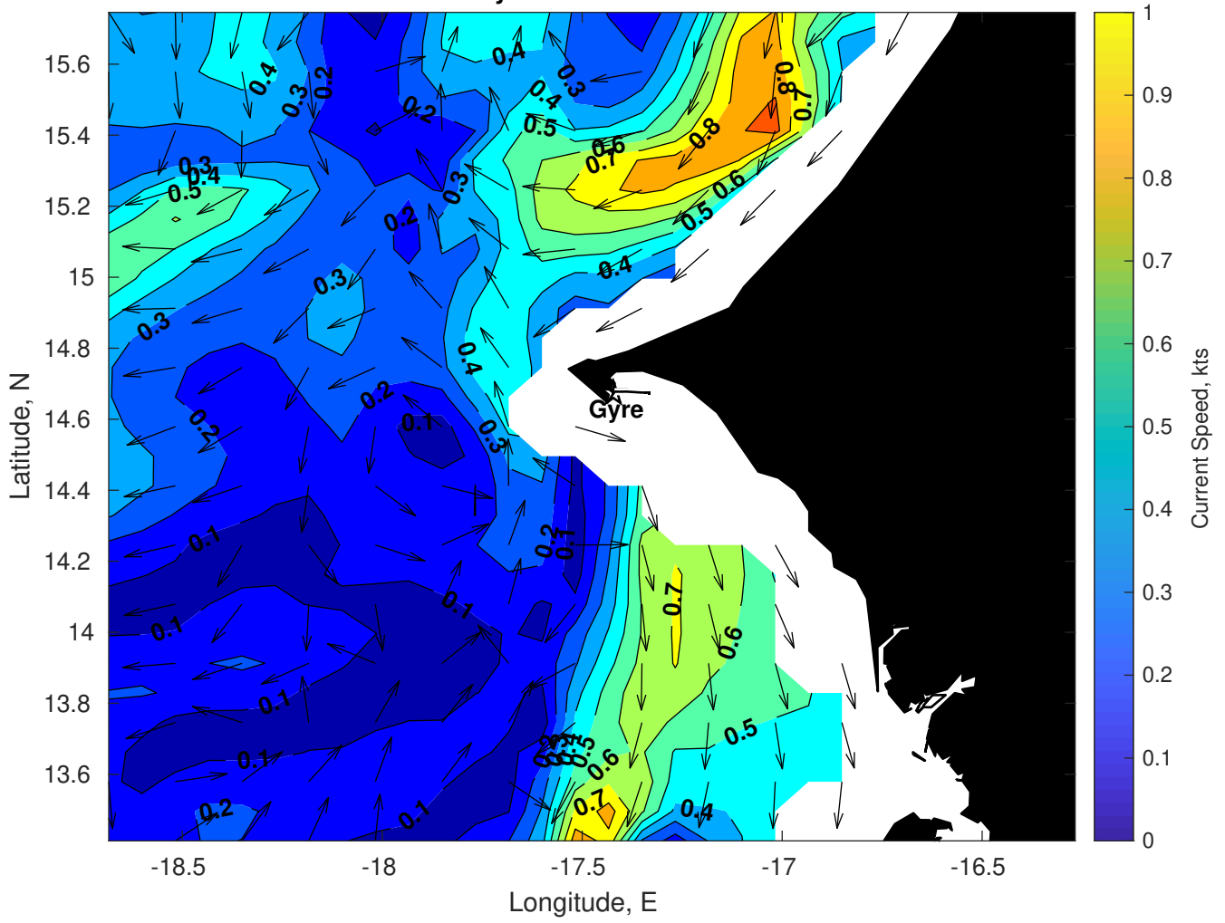
Surface Currents for Gyre at 30-Mar-2025 00:00:00
