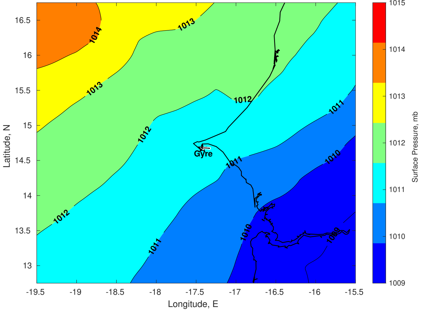
Surface Pressure (mb) for Gyre at 31-Mar-2025 00:00:00
