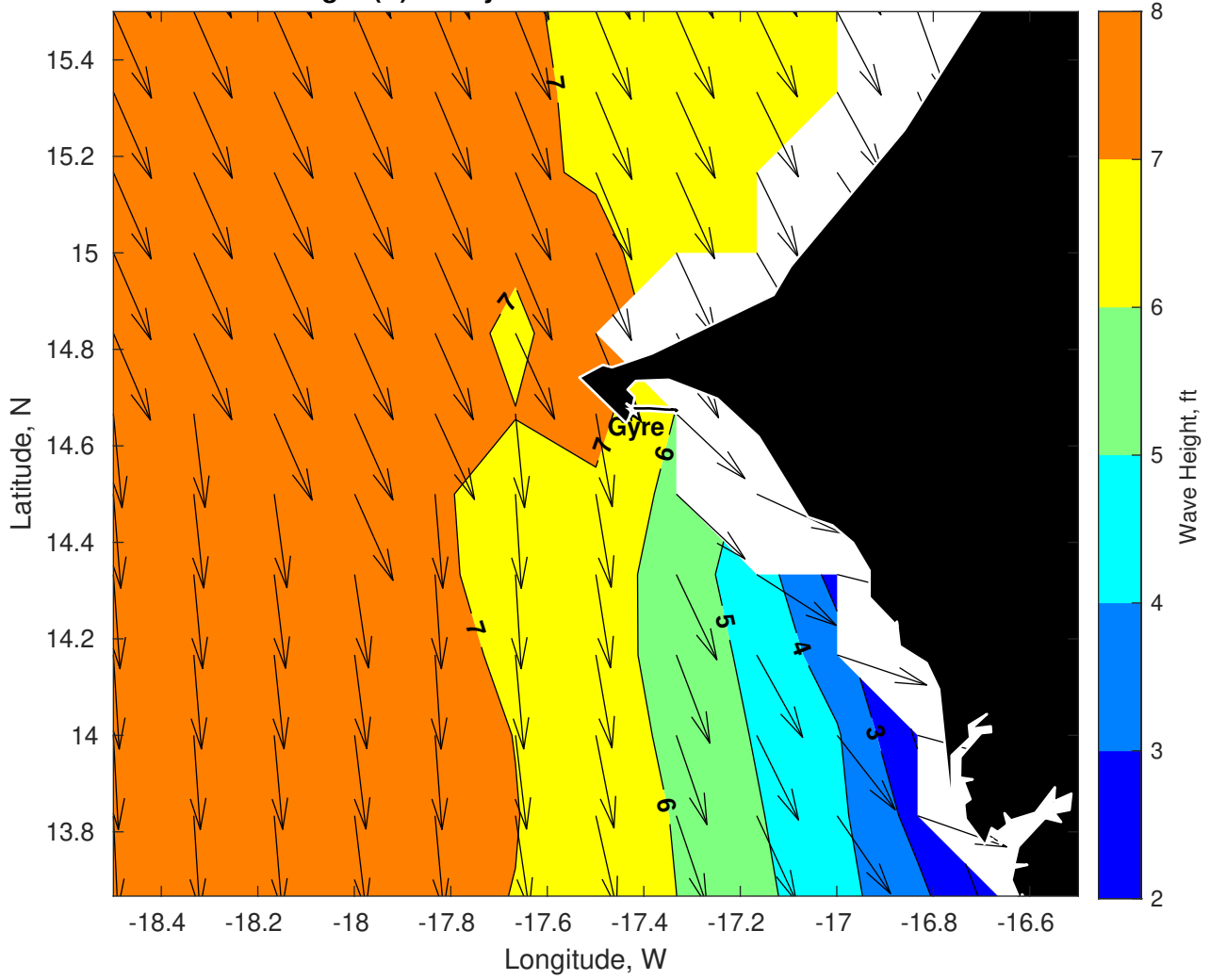
Wave Height (ft) for Gyre at 31-Mar-2025 09:00:00
