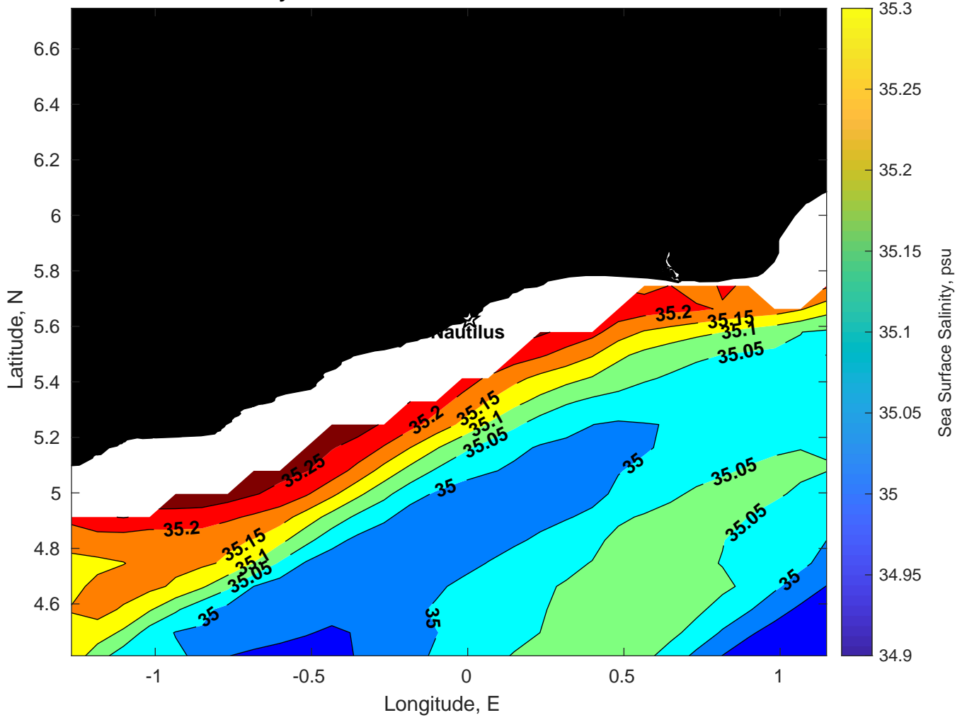
Surface Salinity for Nautilus at 30-Mar-2025 00:00:00
