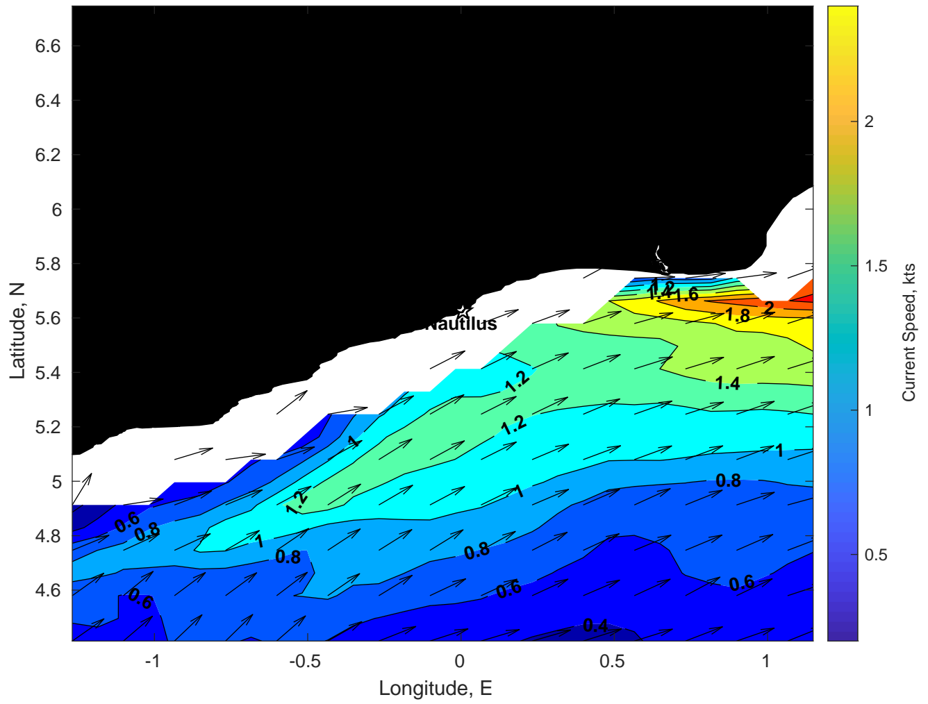
Surface Currents for Nautilus at 30-Mar-2025 00:00:00
