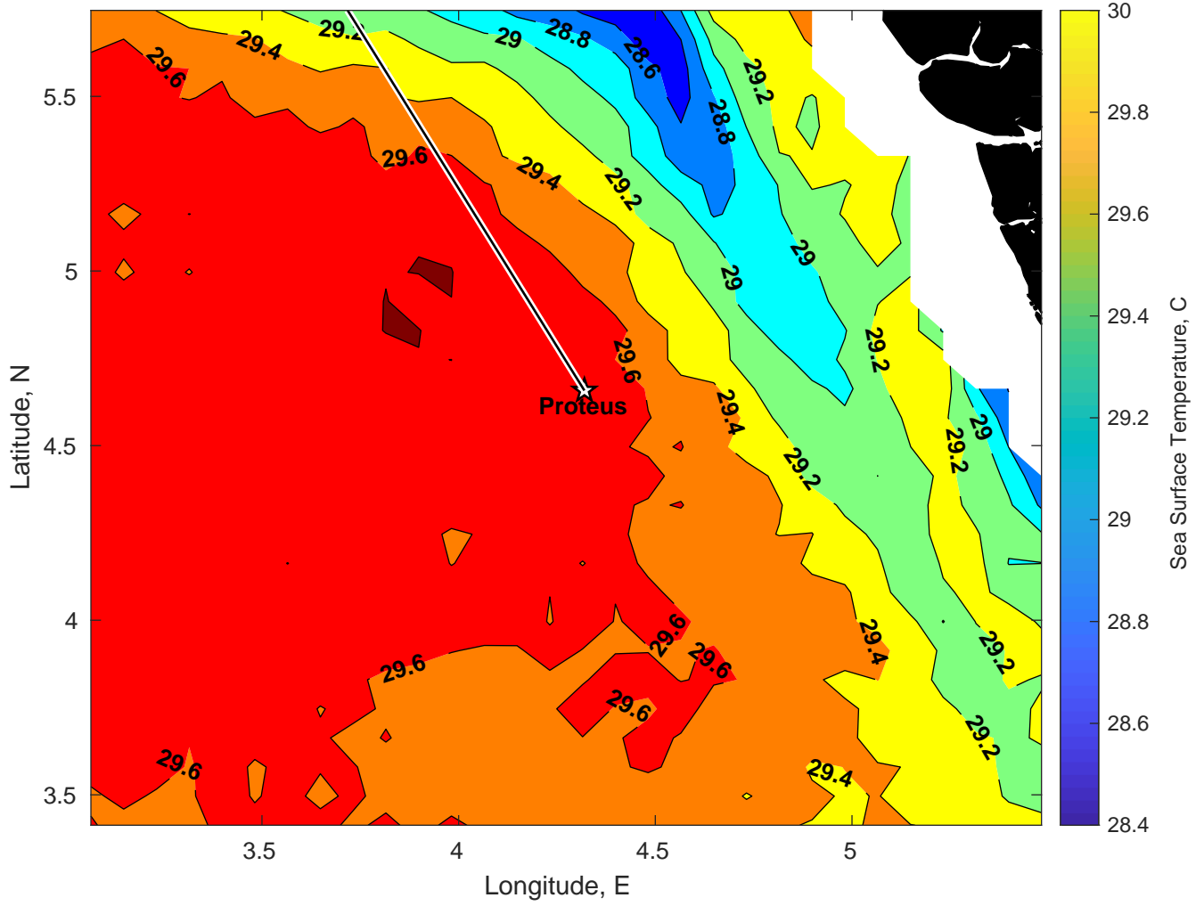
SST for Proteus at 30-Mar-2025 00:00:00
