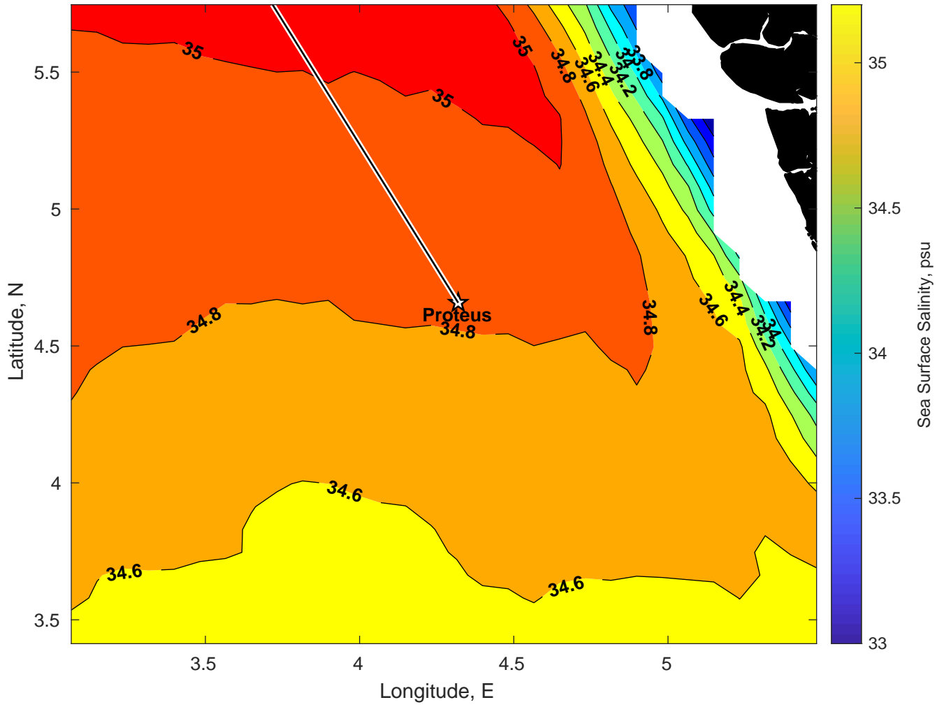
Surface Salinity for Proteus at 30-Mar-2025 00:00:00
