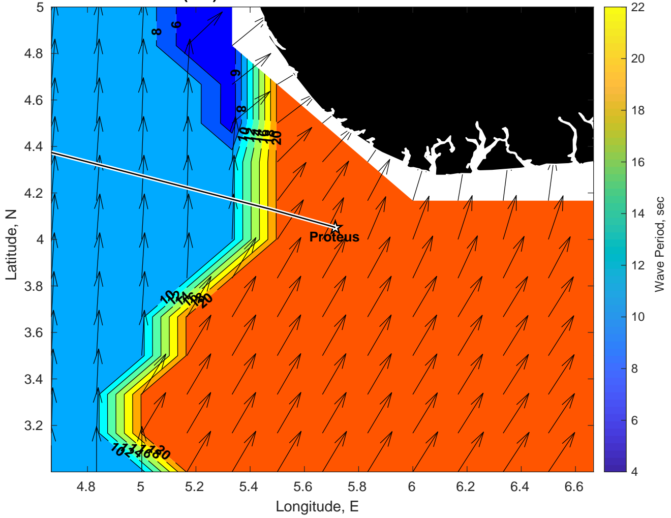
Wave Period (sec) for Proteus at 31-Mar-2025 09:00:00
