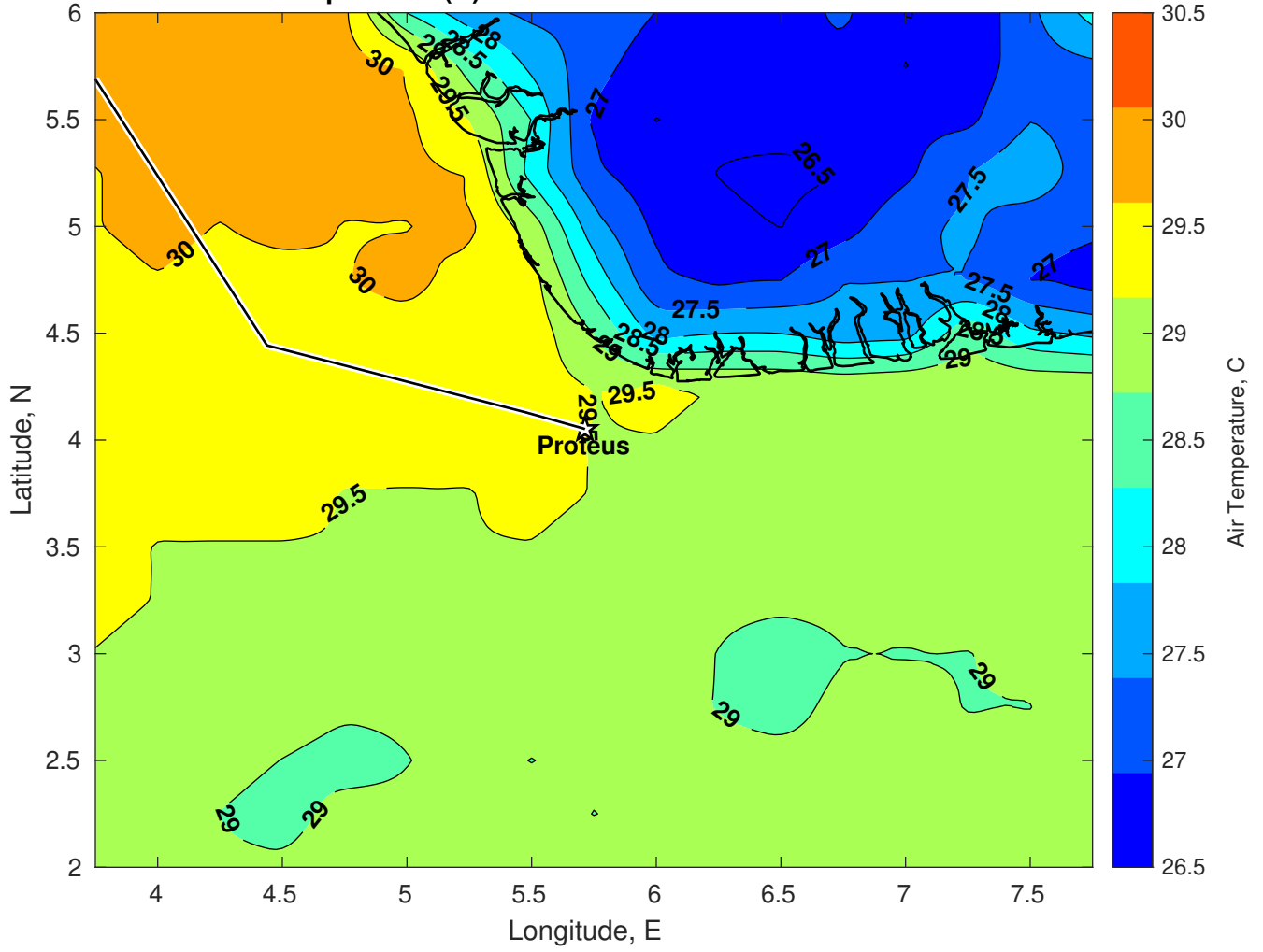
Air Temperature (C) for Proteus at 31-Mar-2025
