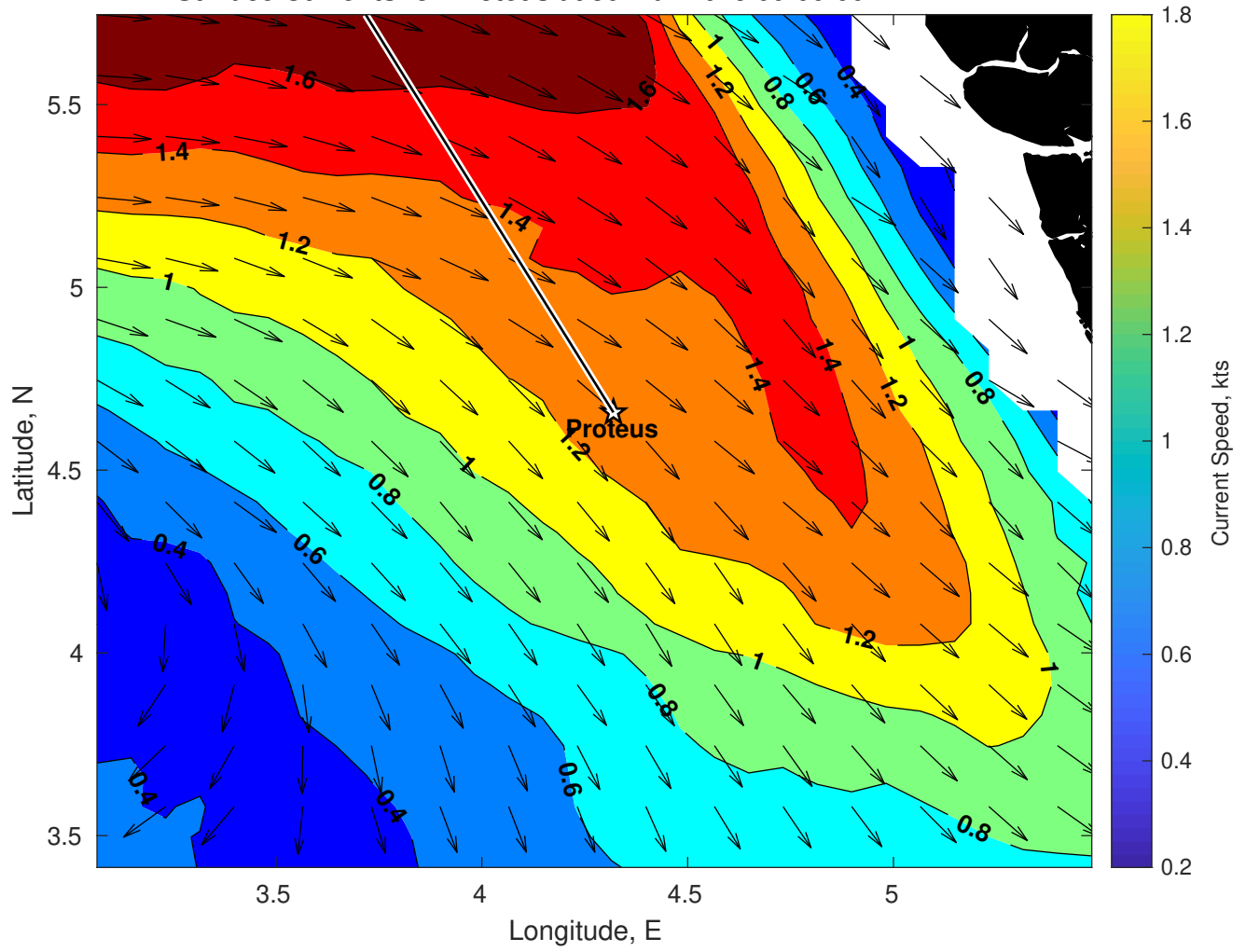
Surface Currents for Proteus at 30-Mar-2025 00:00:00
