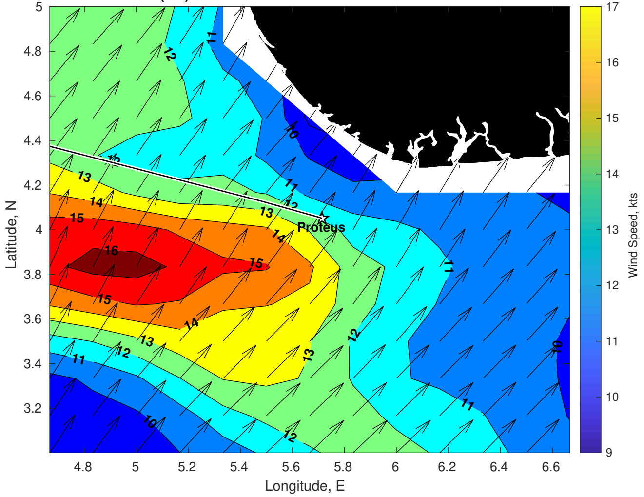
Winds (kts) for Proteus at 31-Mar-2025 09:00:00
