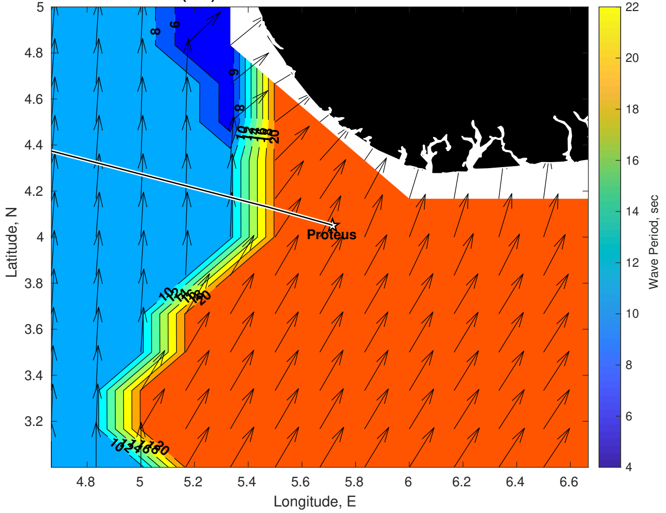
Wave Period (sec) for Proteus at 31-Mar-2025 09:00:00
