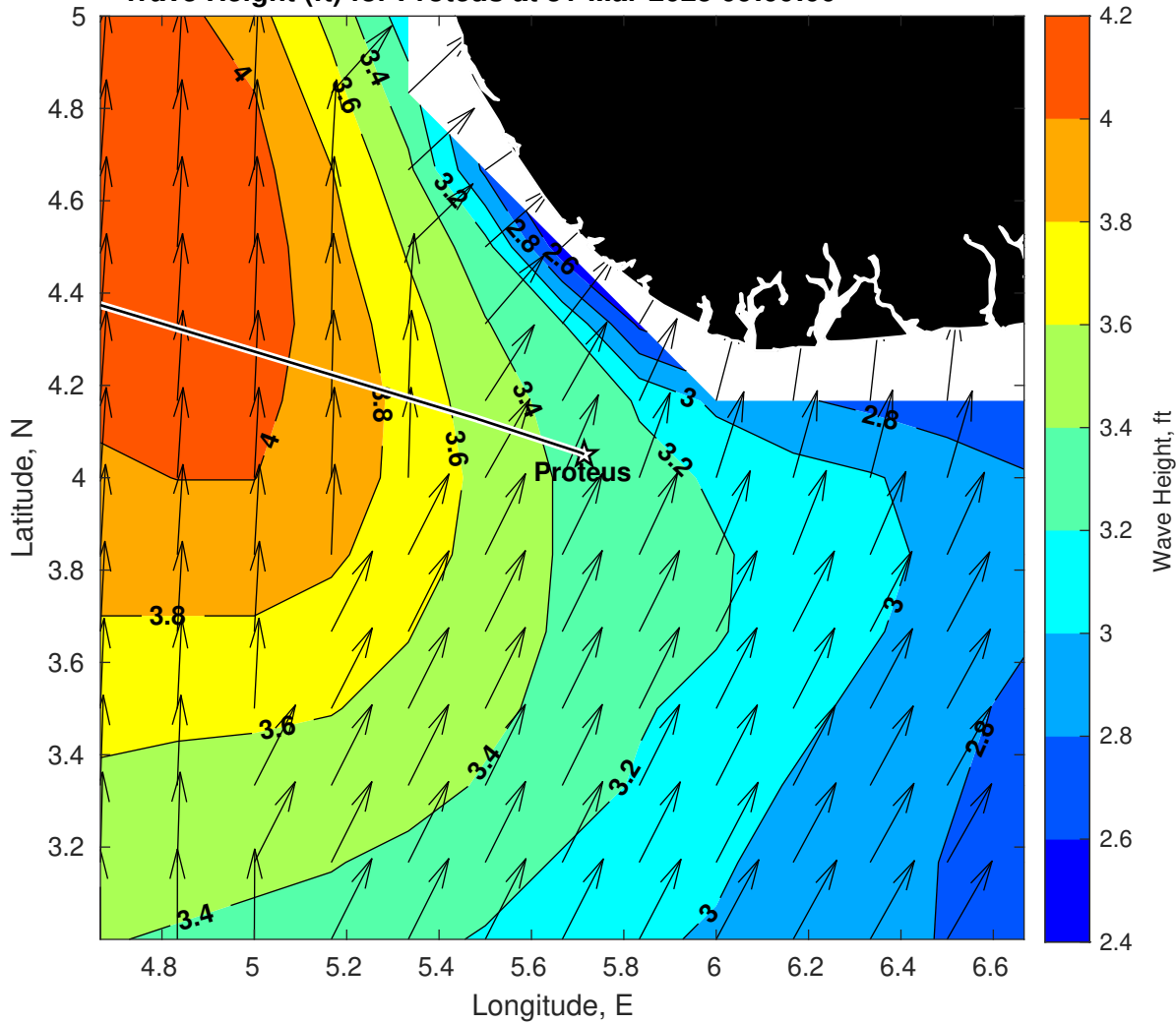
Wave Height (ft) for Proteus at 31-Mar-2025 09:00:00
