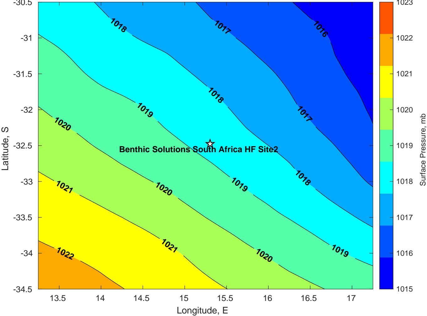
Surface Pressure (mb) for Benthic Solutions South Africa HF Site2 at 02-Apr-2025 00:00:00
