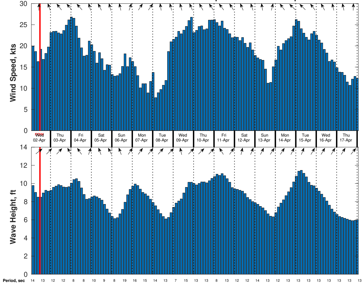
Wind & Wave Forecast for Benthic Solutions South Africa HF Site2 from 01-Apr-2025 02:00:00 to 17-Apr-2025 02:00:00
