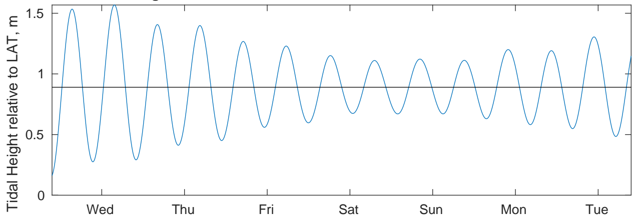
Tidal Currents and Heights for Benthic Solutions South Africa HF Site2 at 20250401
