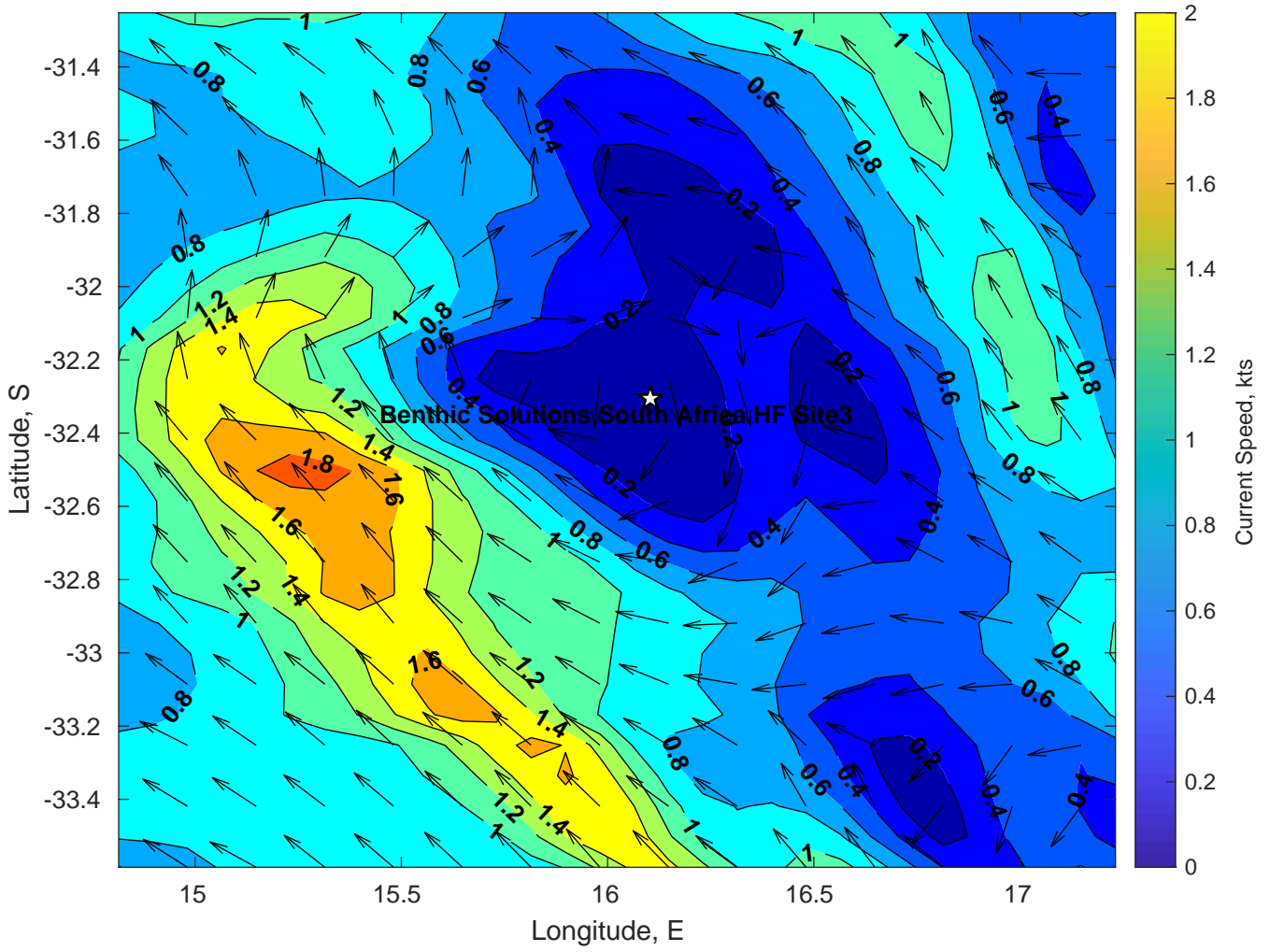
Surface Currents for Benthic Solutions South Africa HF Site3 at 31-Mar-2025 00:00:00
