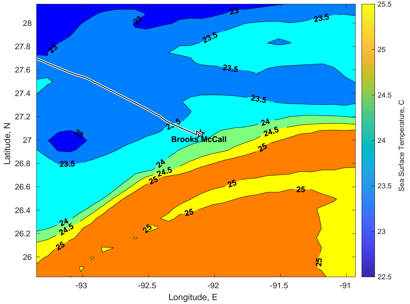
SST for Brooks McCall at 31-Mar-2025 00:00:00
