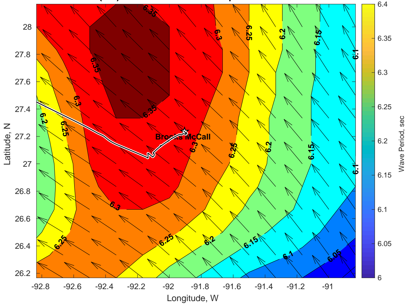
Wave Period (sec) for Brooks McCall at 01-Apr-2025 09:00:00
