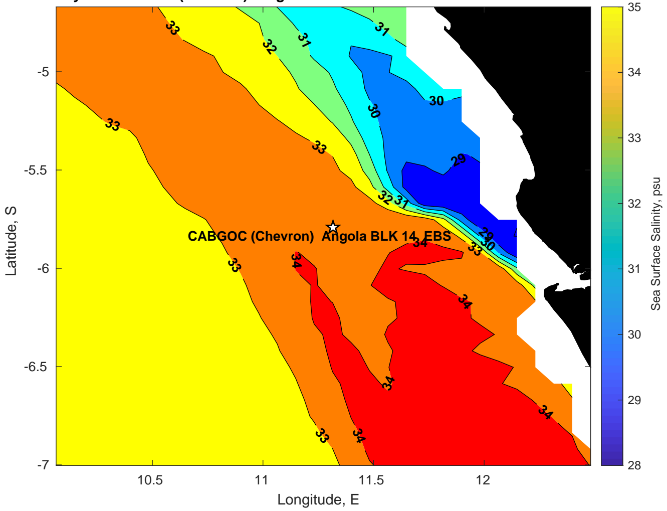
Surface Salinity for CABGOC (Chevron) Angola BLK 14 EBS at 31-Mar-2025 00:00:00
