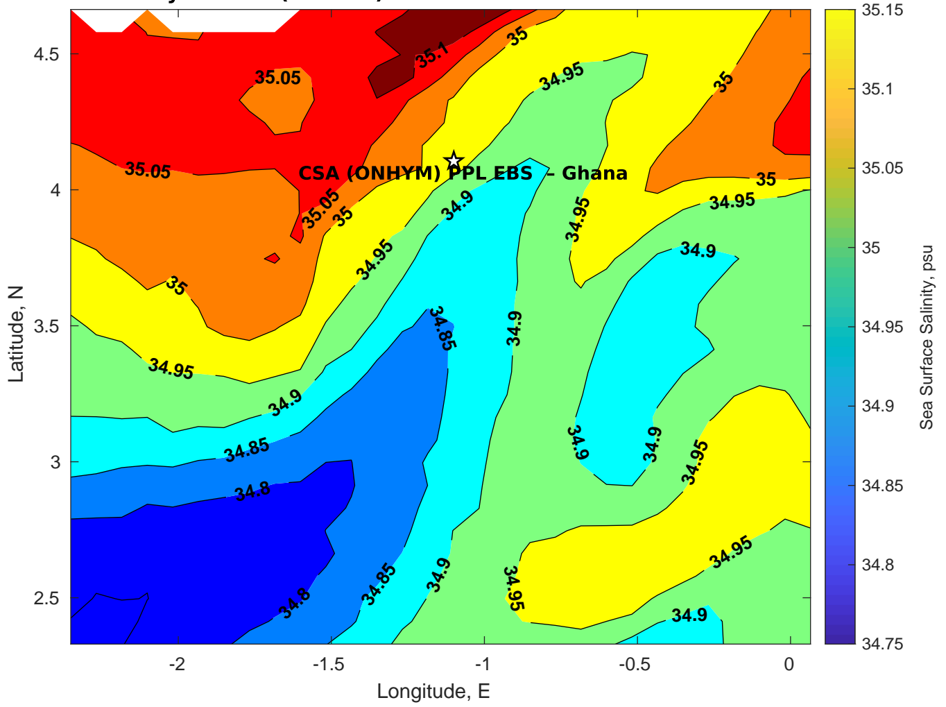
Surface Salinity for CSA (ONHYM) PPL EBS - Ghana at 31-Mar-2025 00:00:00
