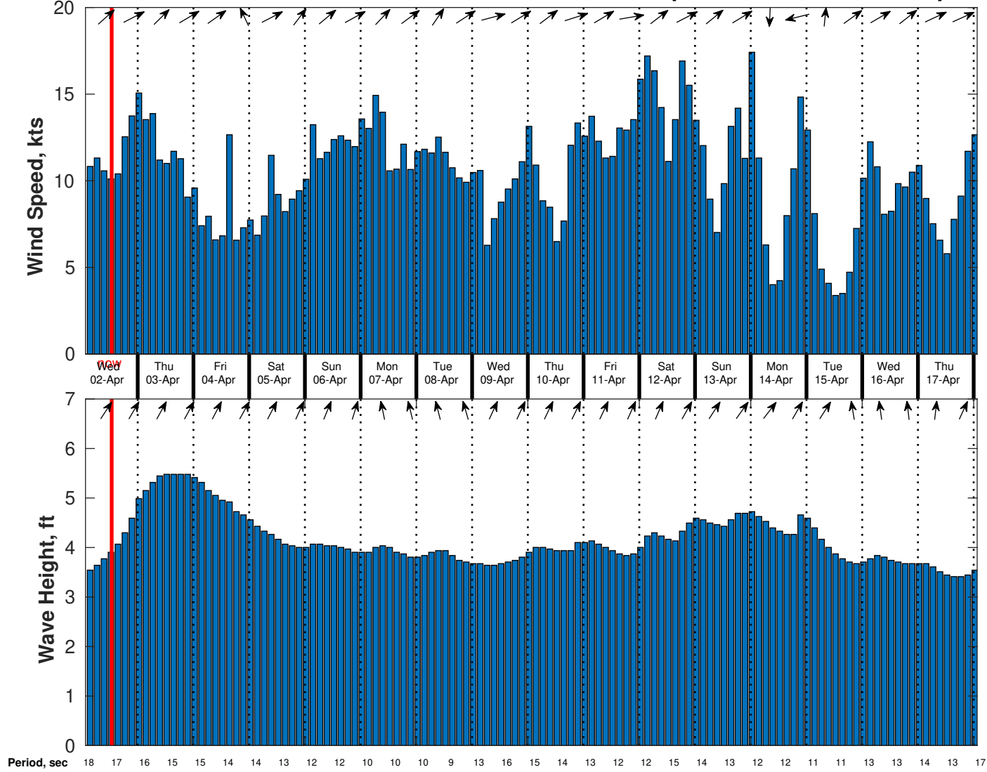
Wind & Wave Forecast for CSA (ONHYM) PPL EBS - Ghana from 01-Apr-2025 02:00:00 to 17-Apr-2025 02:00:00
