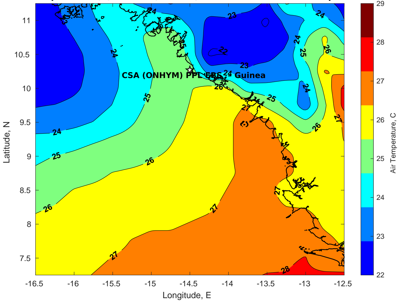
Air Temperature (C) for CSA (ONHYM) PPL EBS - Guinea at 01-Apr-2025
