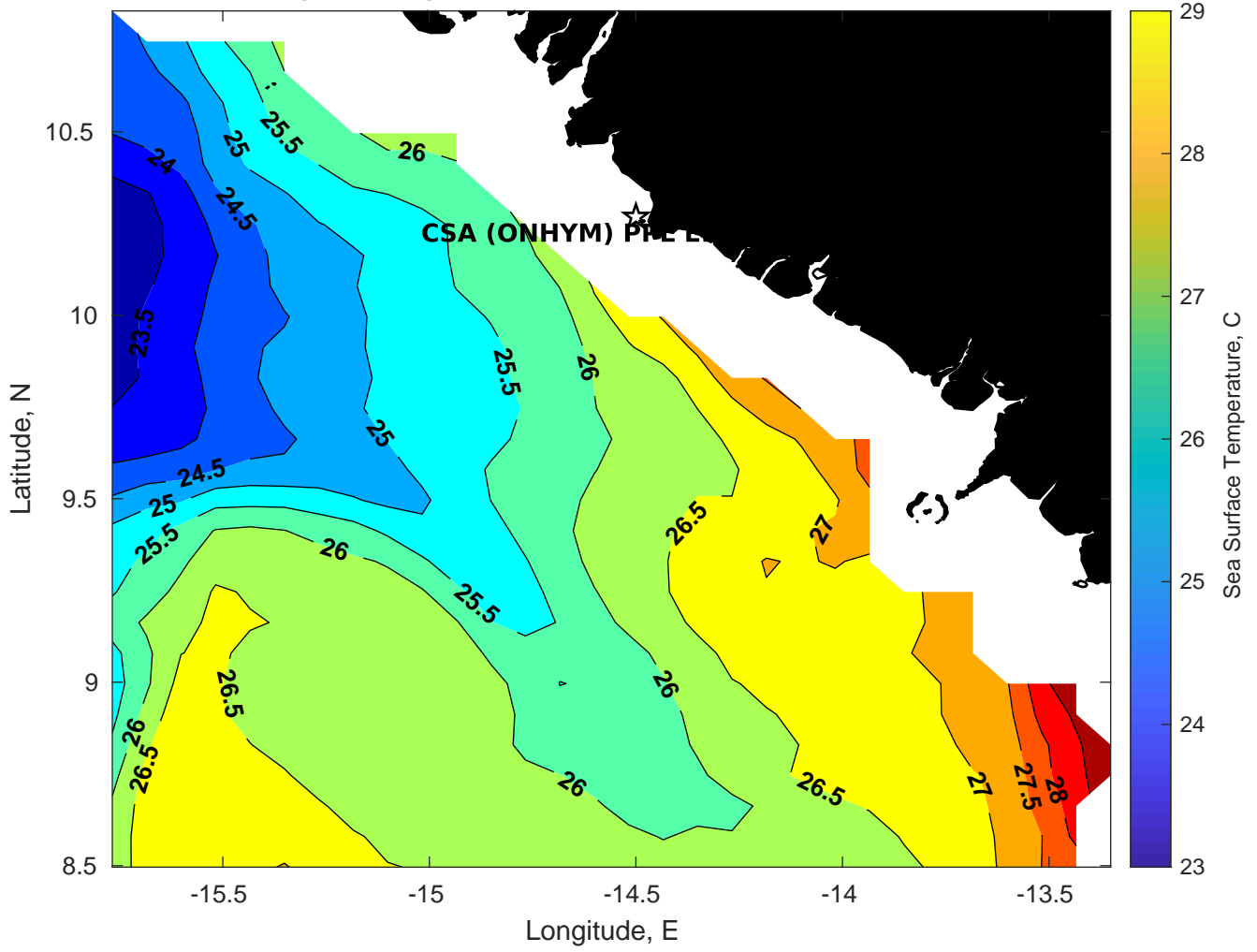
SST for CSA (ONHYM) PPL EBS - Guinea at 31-Mar-2025 00:00:00
