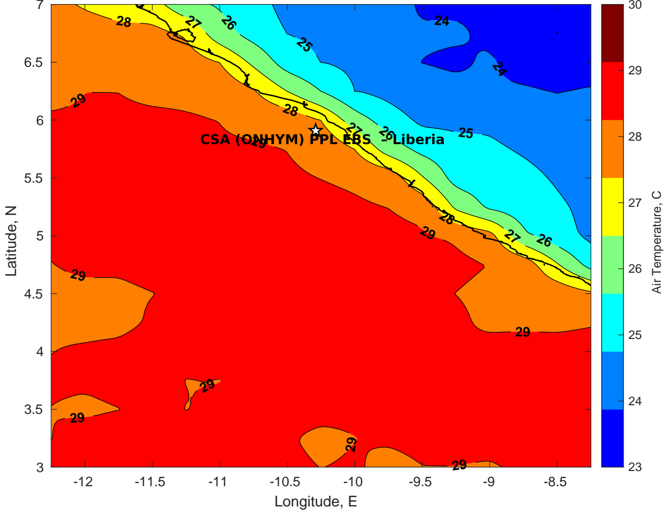
Air Temperature (C) for CSA (ONHYM) PPL EBS - Liberia at 01-Apr-2025
