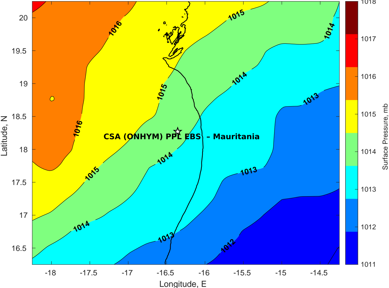
Surface Pressure (mb) for CSA (ONHYM) PPL EBS - Mauritania at 01-Apr-2025 00:00:00
