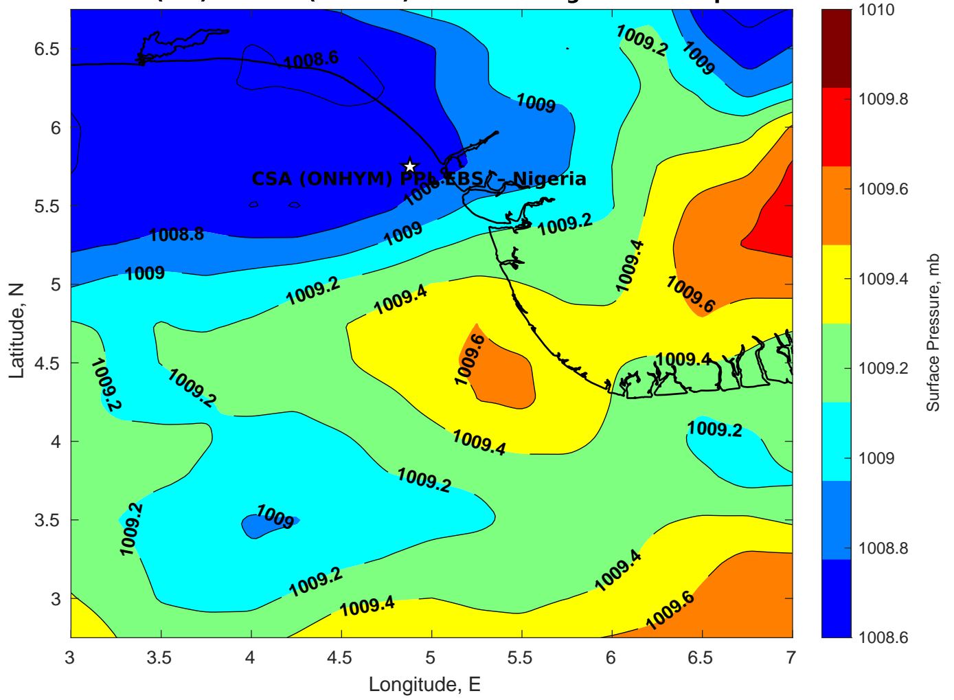
Surface Pressure (mb) for CSA (ONHYM) PPL EBS - Nigeria at 01-Apr-2025 00:00:00
