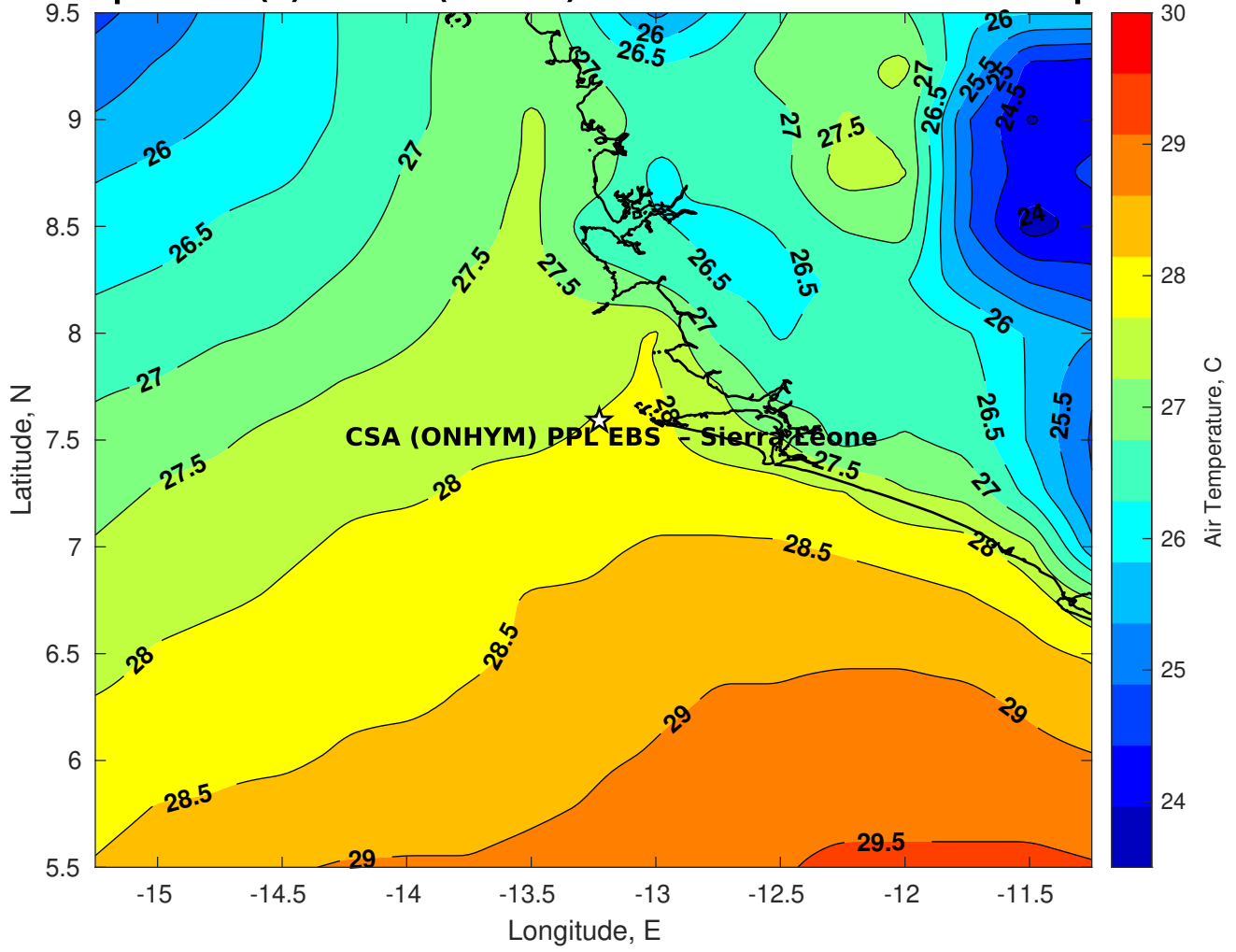
Air Temperature (C) for CSA (ONHYM) PPL EBS - Sierra Leone at 01-Apr-2025
