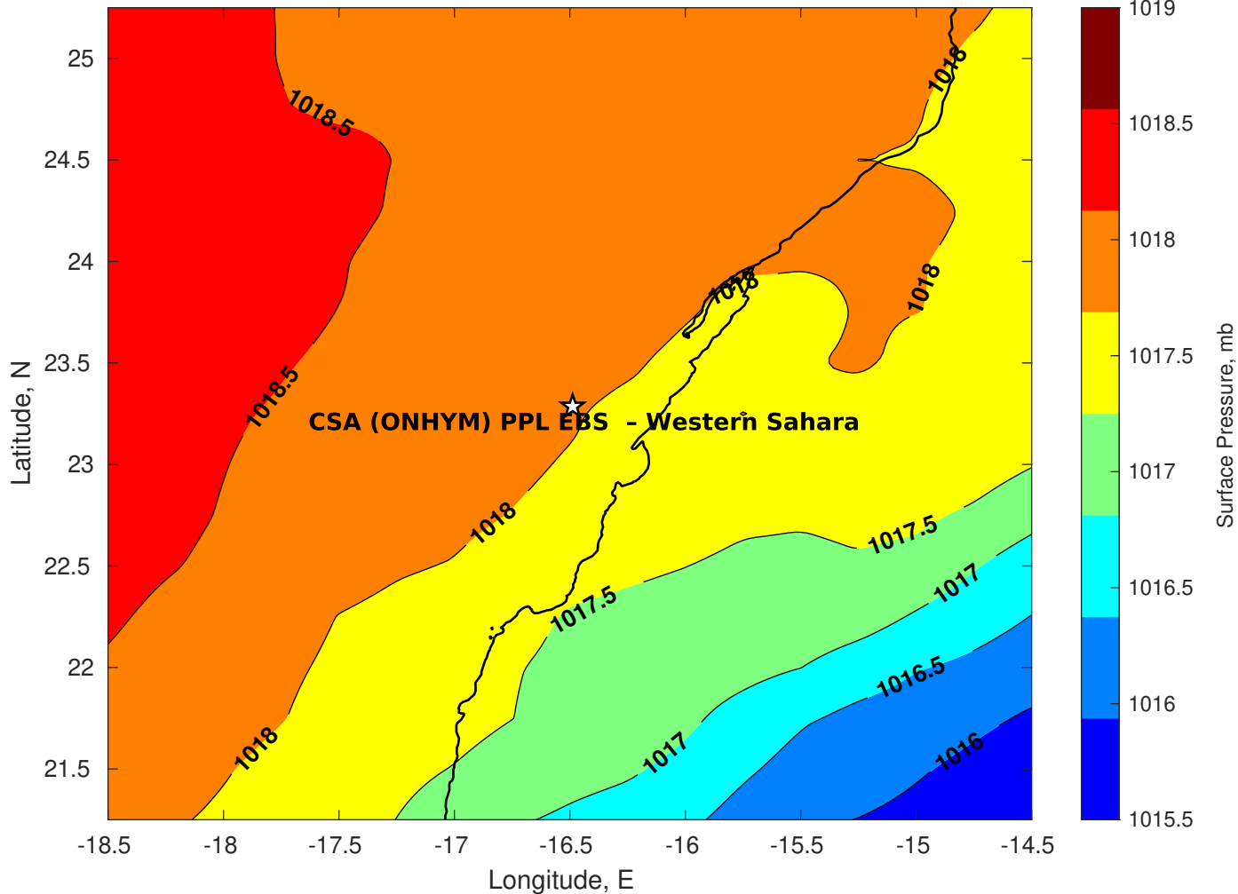
Surface Pressure (mb) for CSA (ONHYM) PPL EBS - Western Sahara at 01-Apr-2025 00:00:00
