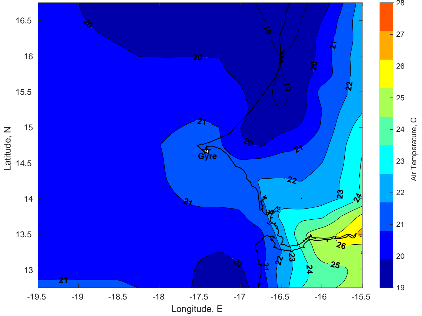
Air Temperature (C) for Gyre at 01-Apr-2025
