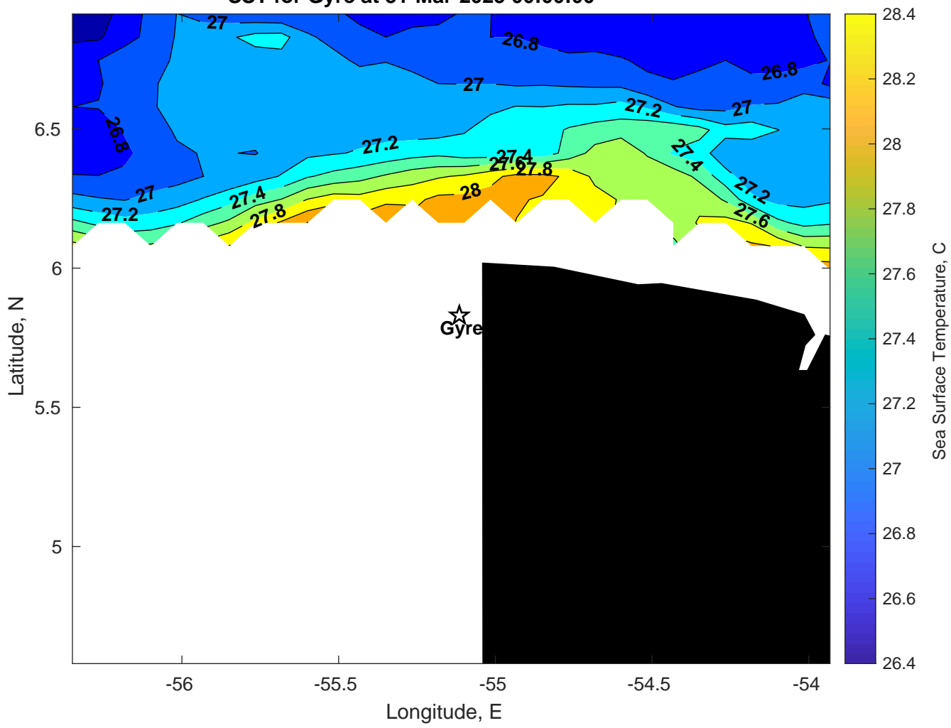
SST for Gyre at 31-Mar-2025 00:00:00
