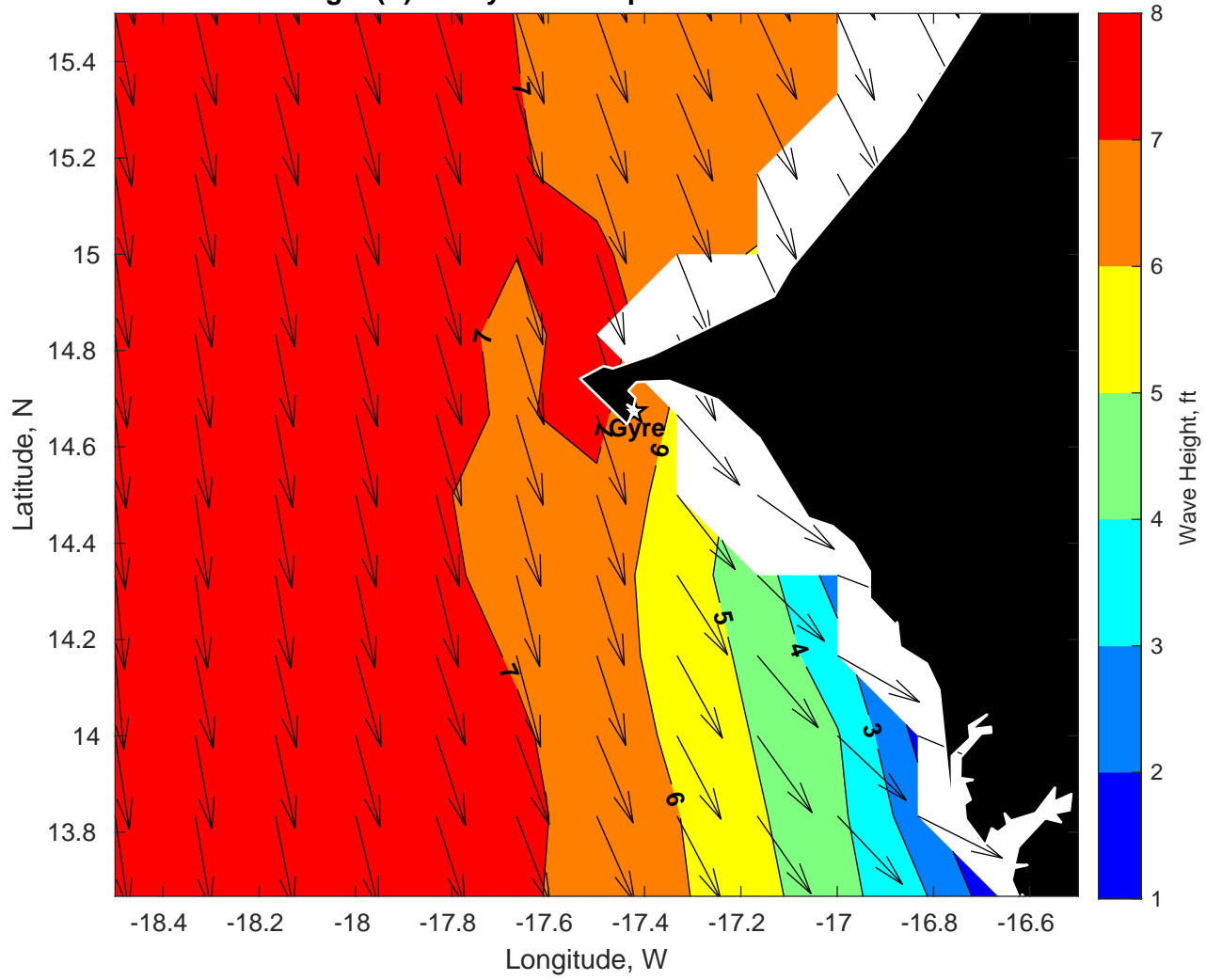
Wave Height (ft) for Gyre at 01-Apr-2025 09:00:00
