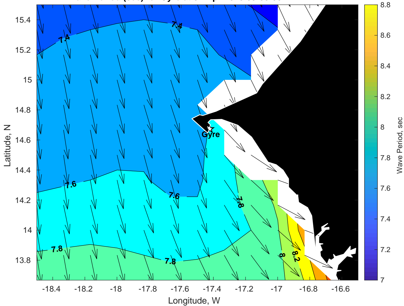
Wave Period (sec) for Gyre at 01-Apr-2025 09:00:00
