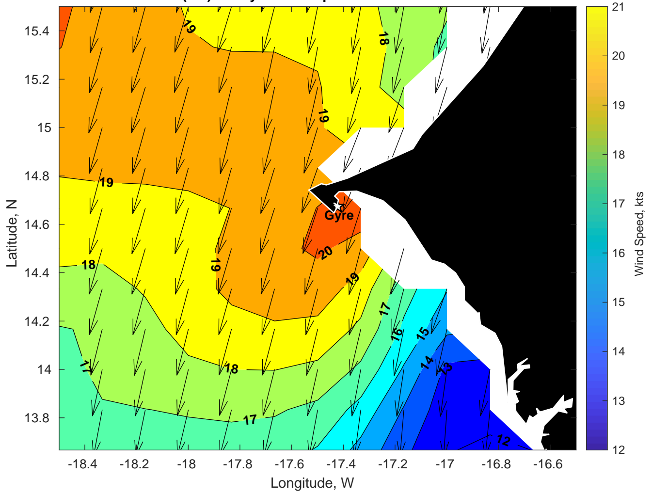
Winds (kts) for Gyre at 01-Apr-2025 09:00:00
