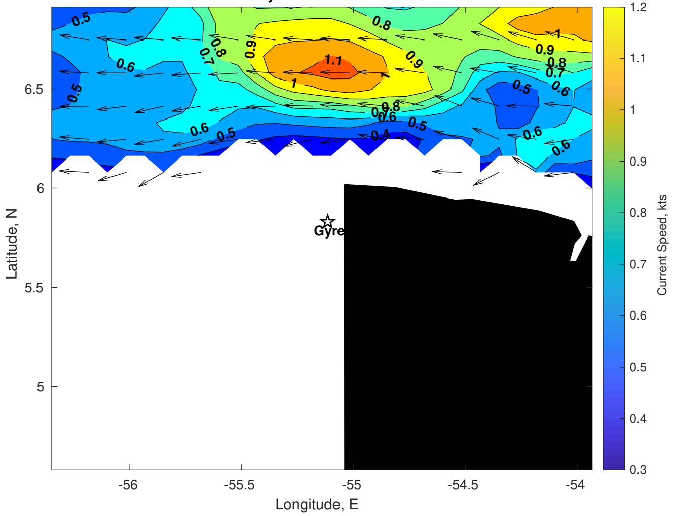
Surface Currents for Gyre at 31-Mar-2025 00:00:00
