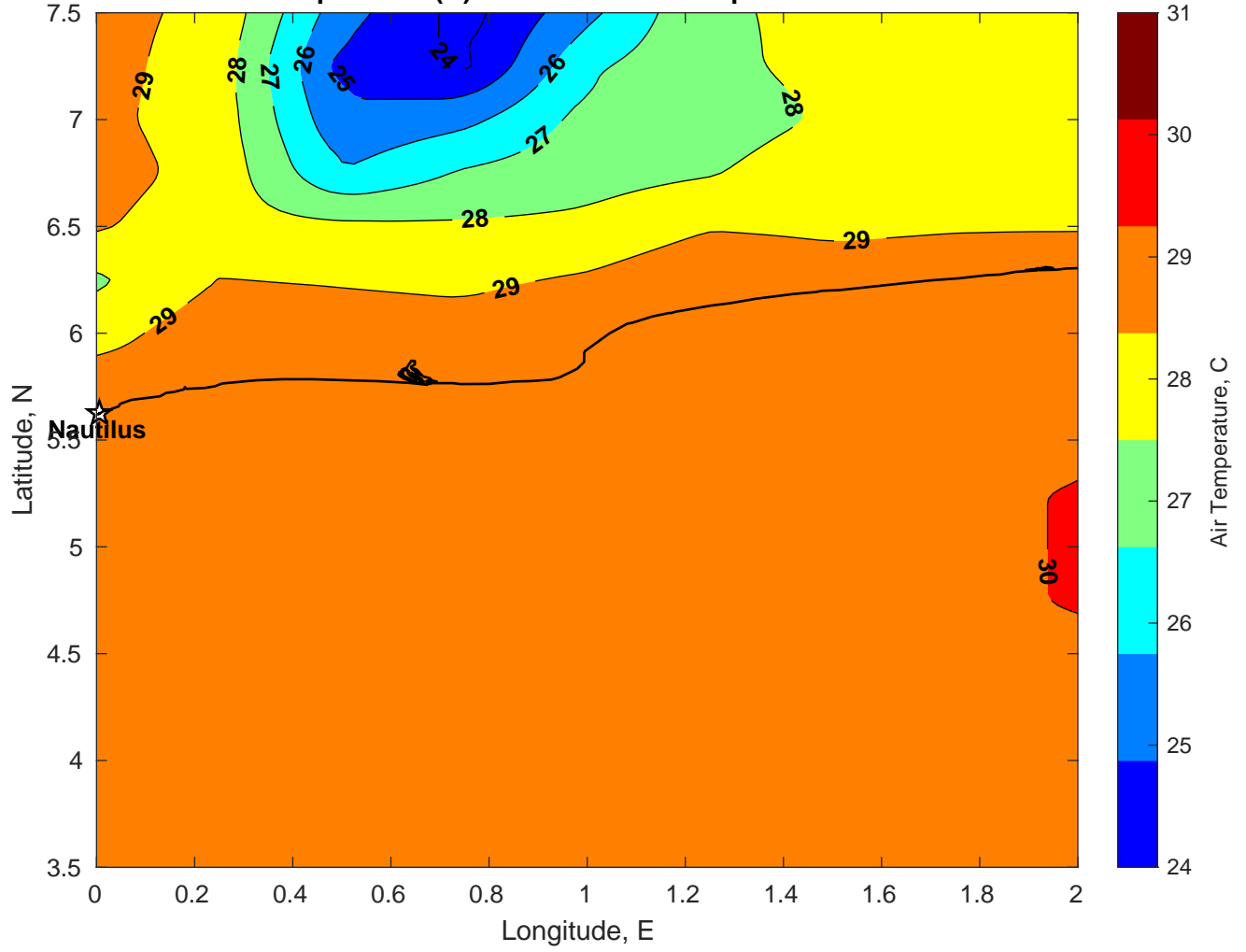
Air Temperature (C) for Nautilus at 01-Apr-2025
