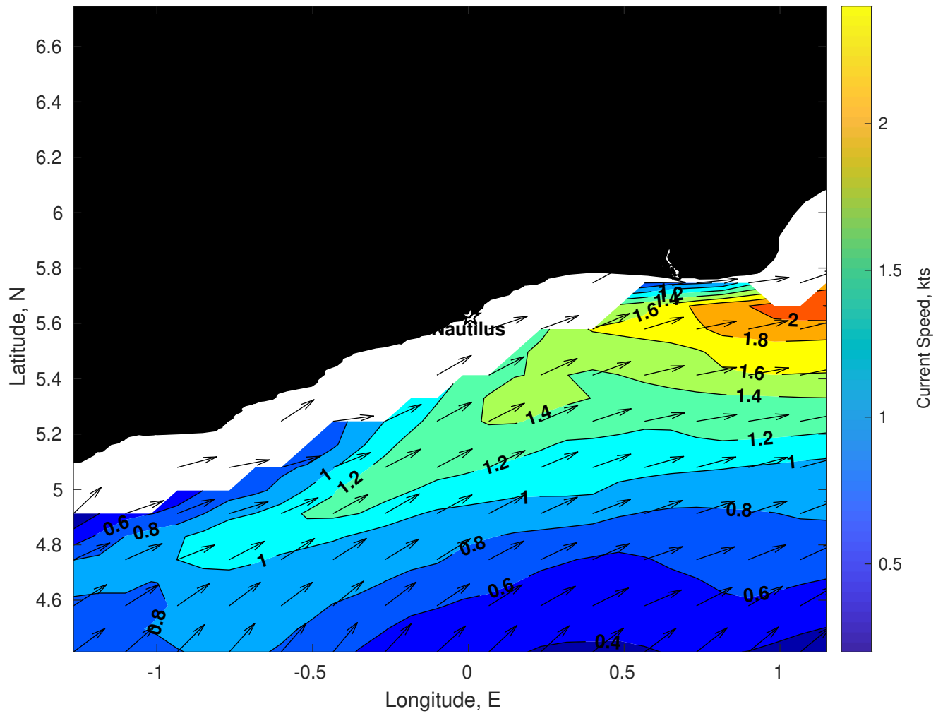
Surface Currents for Nautilus at 31-Mar-2025 00:00:00
