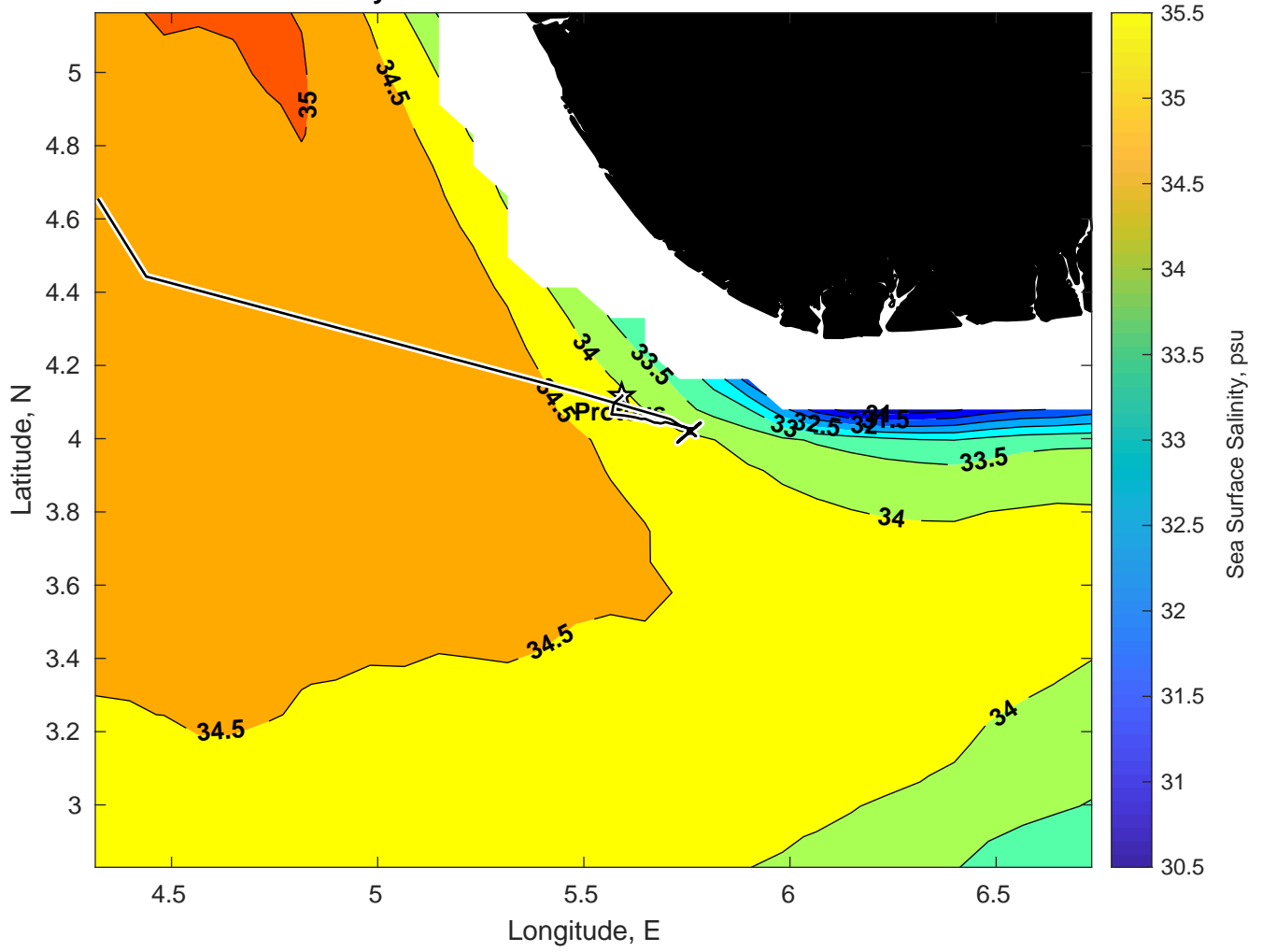
Surface Salinity for Proteus at 31-Mar-2025 00:00:00
