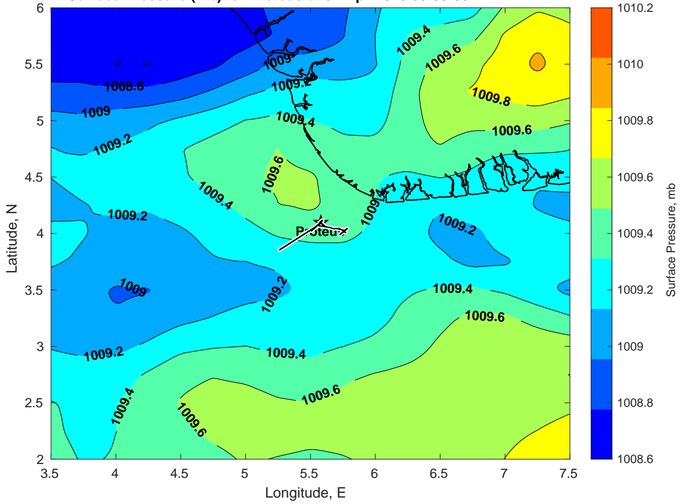
Surface Pressure (mb) for Proteus at 01-Apr-2025 00:00:00
