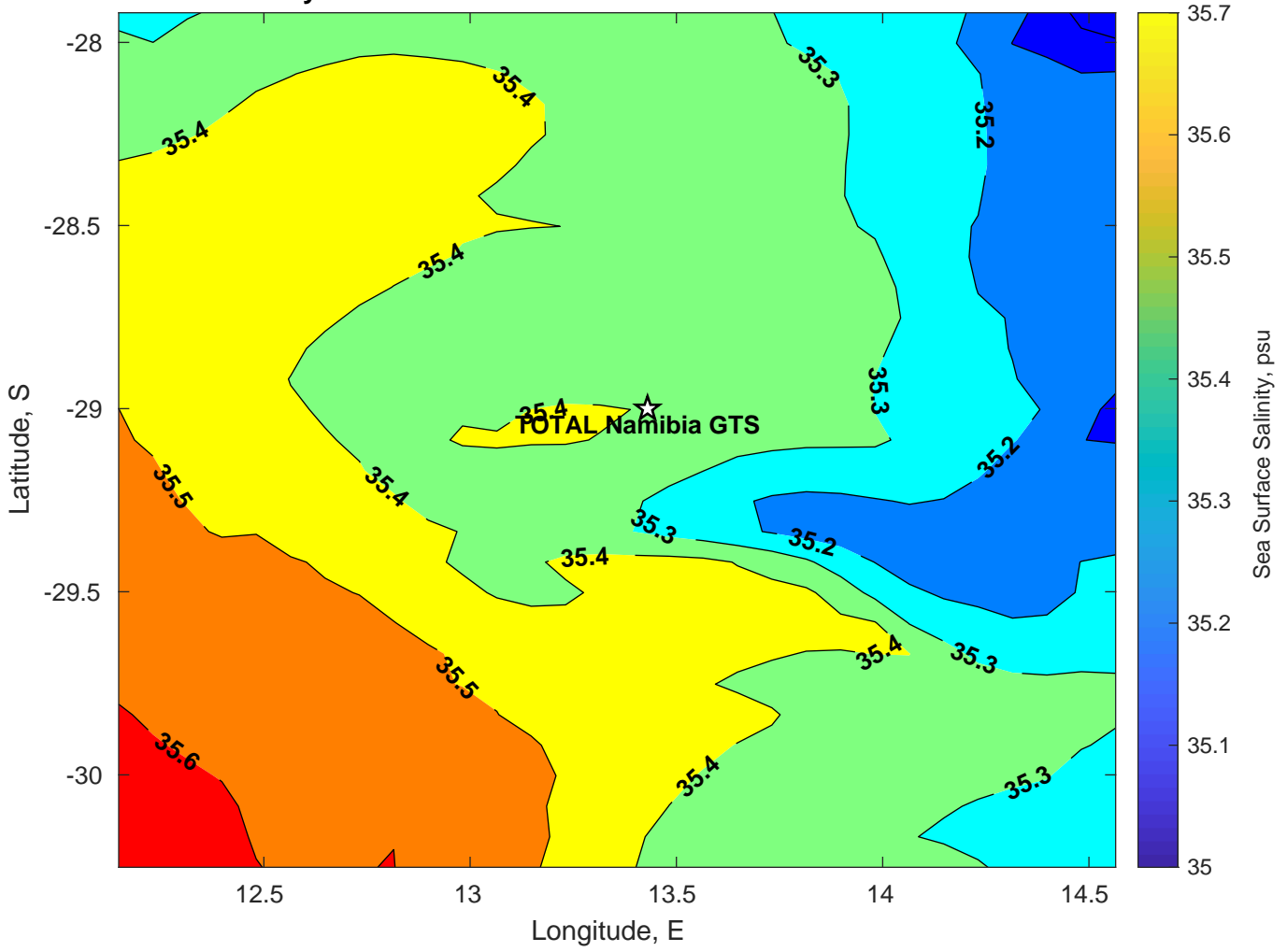
Surface Salinity for TOTAL Namibia GTS at 31-Mar-2025 00:00:00
