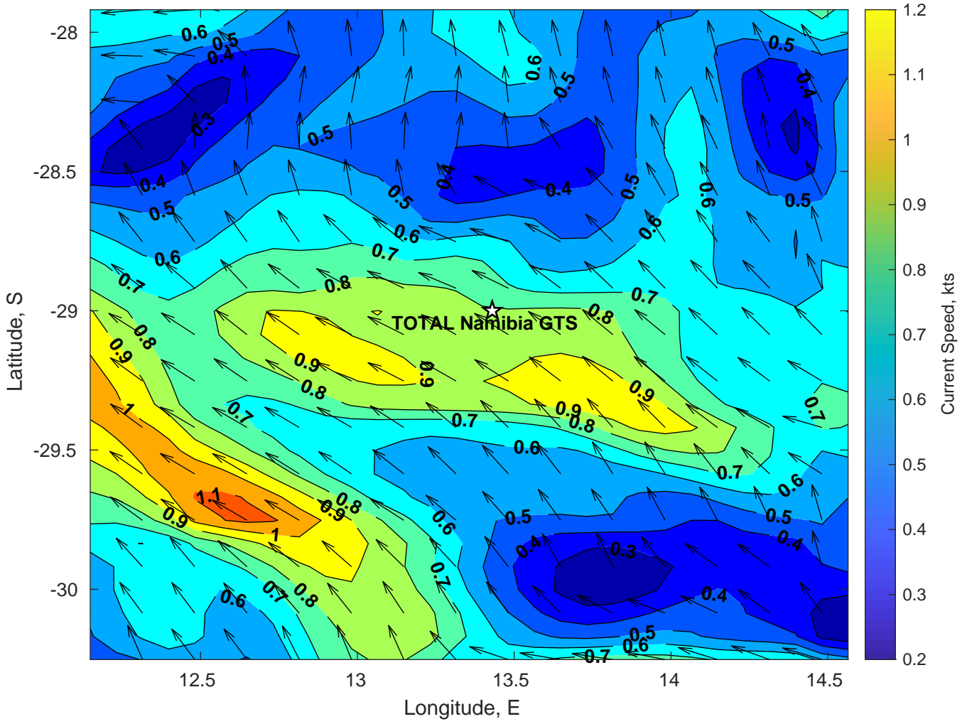
Surface Currents for TOTAL Namibia GTS at 31-Mar-2025 00:00:00
