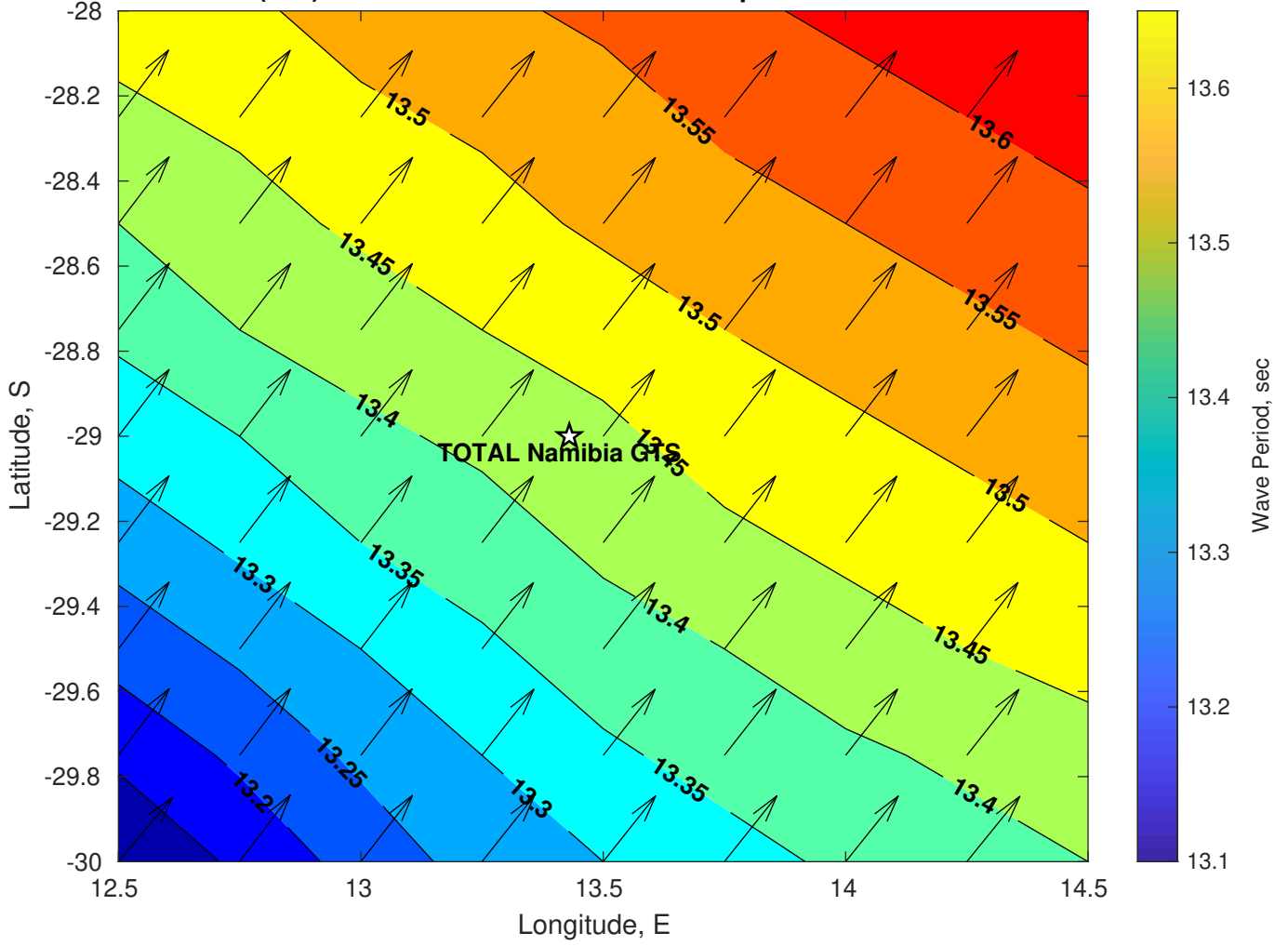
Wave Period (sec) for TOTAL Namibia GTS at 01-Apr-2025 09:00:00
