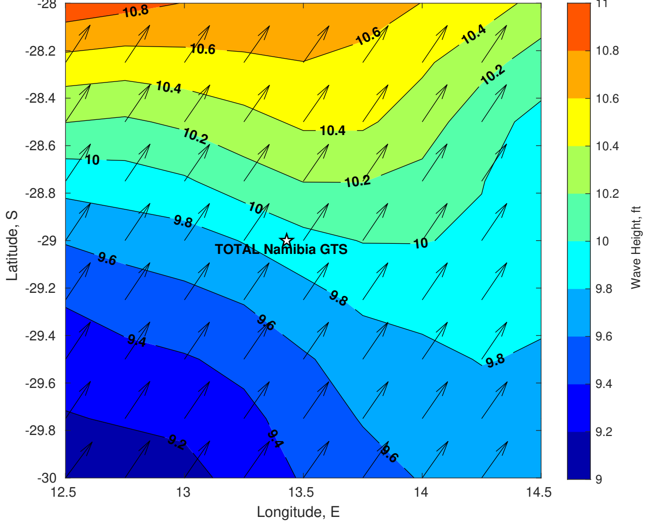
Wave Height (ft) for TOTAL Namibia GTS at 01-Apr-2025 09:00:00
