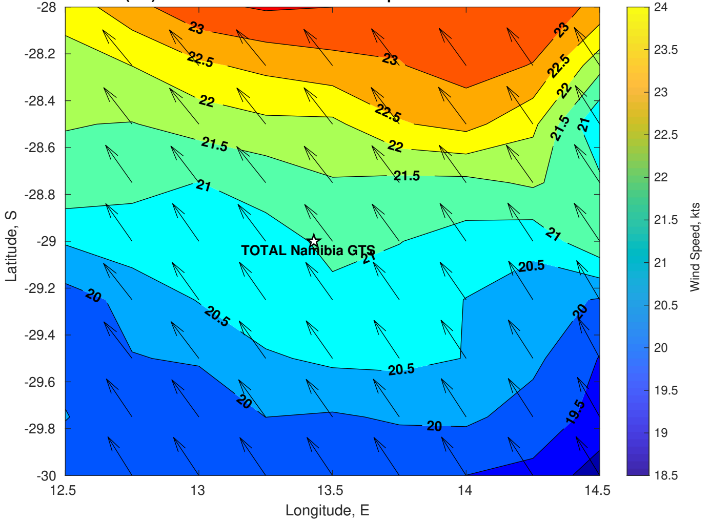
Winds (kts) for TOTAL Namibia GTS at 01-Apr-2025 09:00:00
