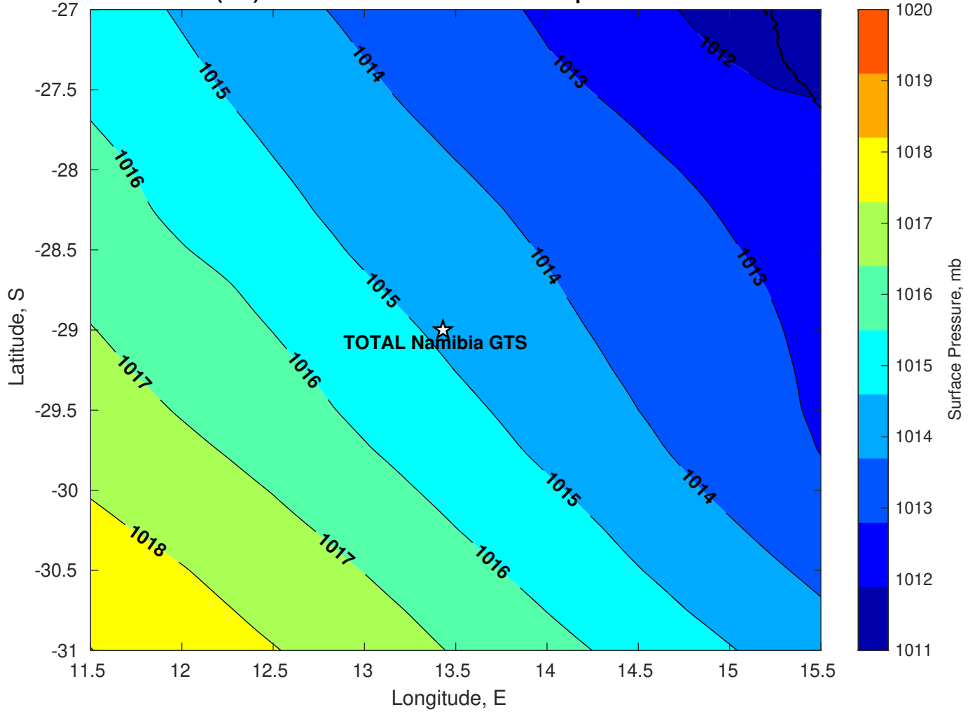
Surface Pressure (mb) for TOTAL Namibia GTS at 03-Apr-2025 00:00:00
