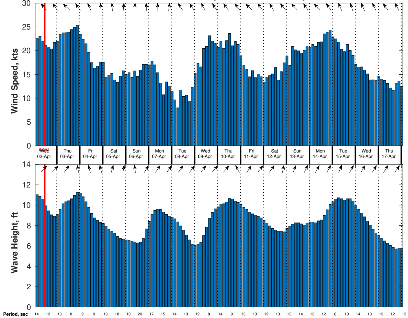
Wind & Wave Forecast for TOTAL Namibia GTS from 01-Apr-2025 02:00:00 to 17-Apr-2025 02:00:00
