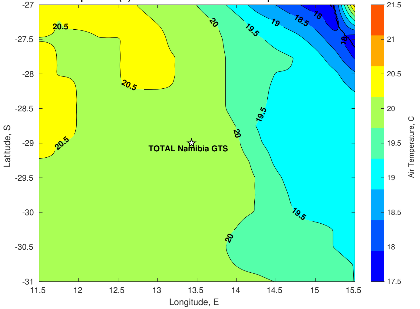
Air Temperature (C) for TOTAL Namibia GTS at 01-Apr-2025
