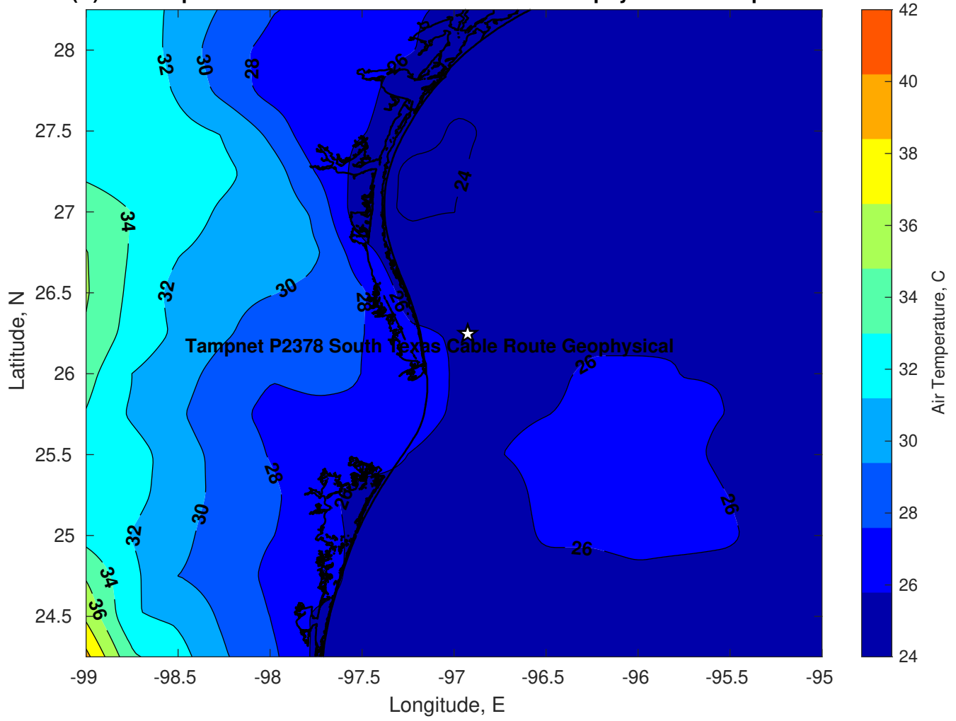
Air Temperature (C) for Tampnet P2378 South Texas Cable Route Geophysical at 01-Apr-2025
