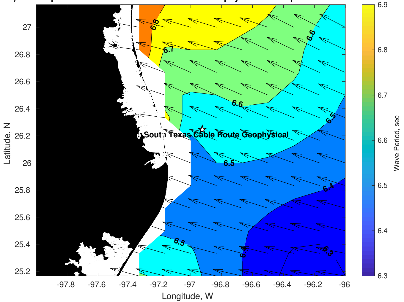
Period (sec) for Tampnet P2378 South Texas Cable Route Geophysical at 01-Apr-2025 09:00:00
