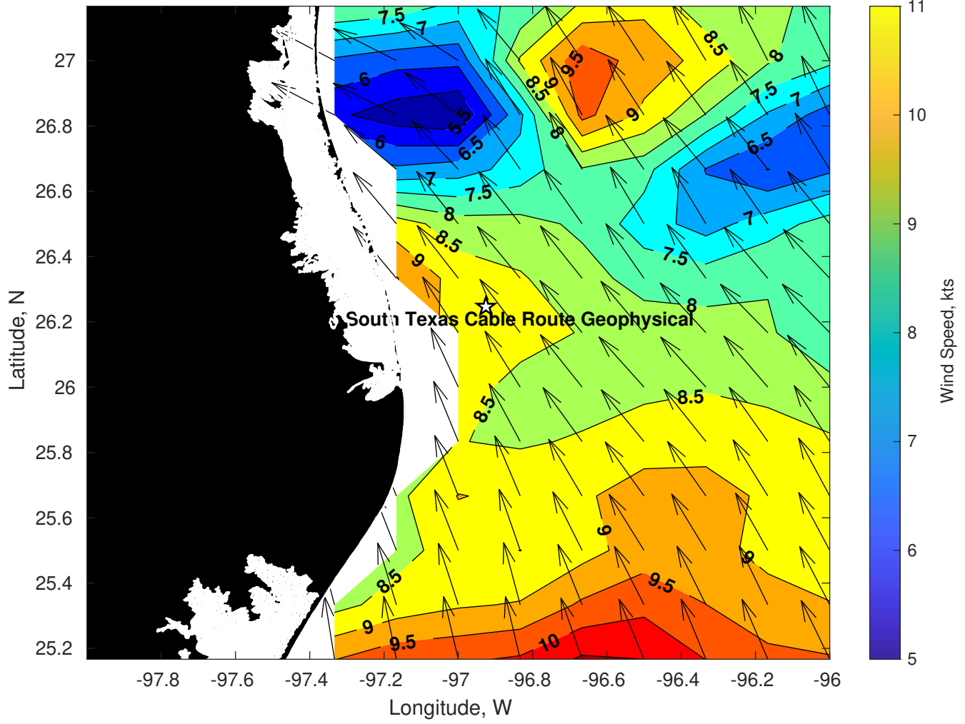
Winds (kts) for Tampnet P2378 South Texas Cable Route Geophysical at 01-Apr-2025 09:00:00
