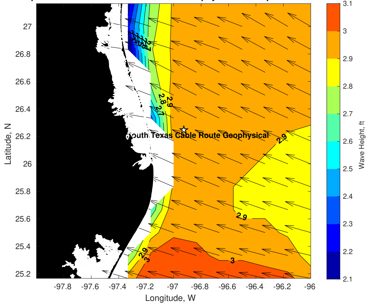
Wave Height (ft) for Tampnet P2378 South Texas Cable Route Geophysical at 01-Apr-2025 09:00:00
