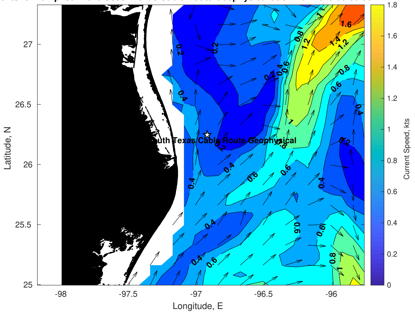
Surface Currents for Tampnet P2378 South Texas Cable Route Geophysical at 31-Mar-2025 00:00:00
