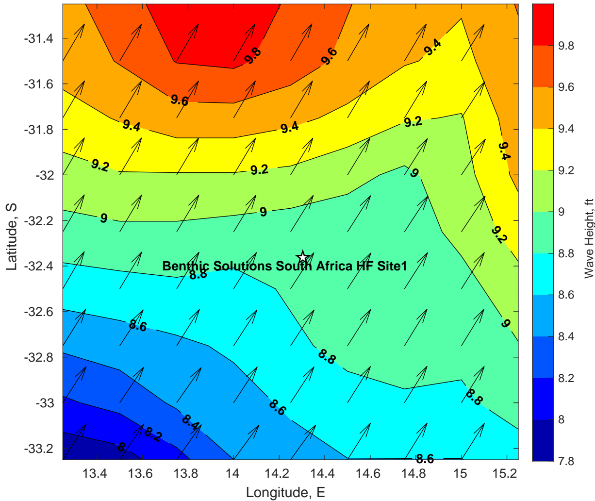
Wave Height (ft) for Benthic Solutions South Africa HF Site1 at 02-Apr-2025 09:00:00
