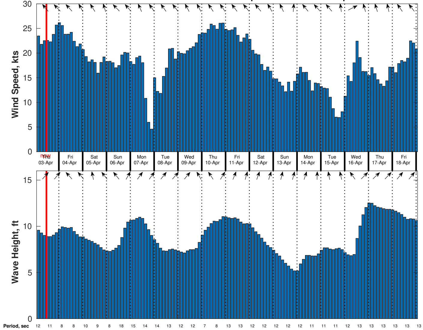
Wind & Wave Forecast for Benthic Solutions South Africa HF Site1 from 02-Apr-2025 02:00:00 to 18-Apr-2025 02:00:00
