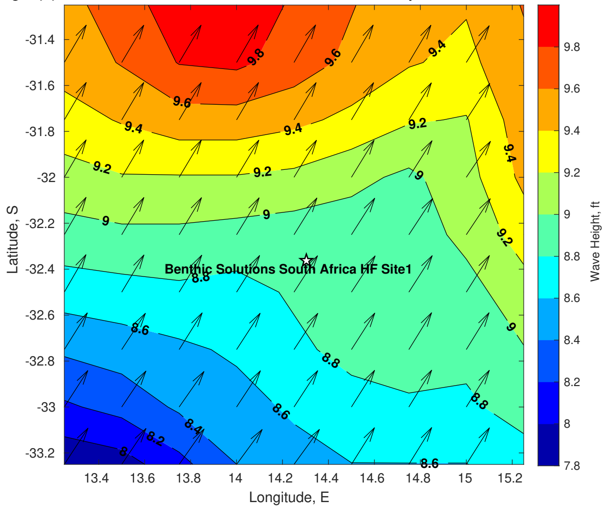
Wave Height (ft) for Benthic Solutions South Africa HF Site1 at 02-Apr-2025 09:00:00
