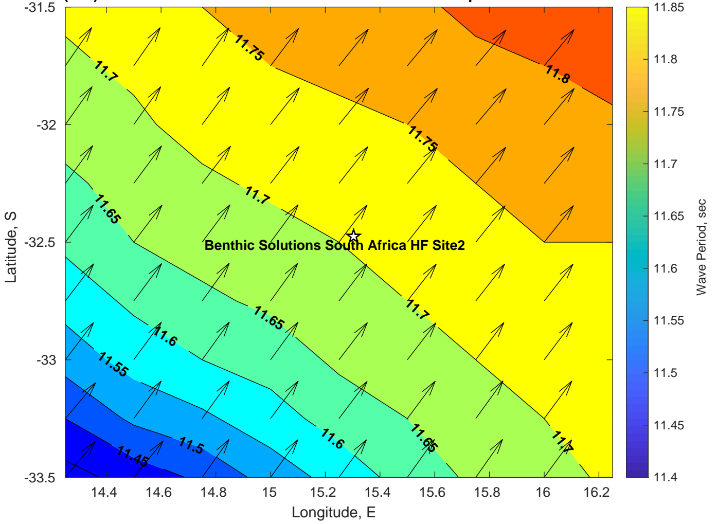
Wave Period (sec) for Benthic Solutions South Africa HF Site2 at 02-Apr-2025 09:00:00
