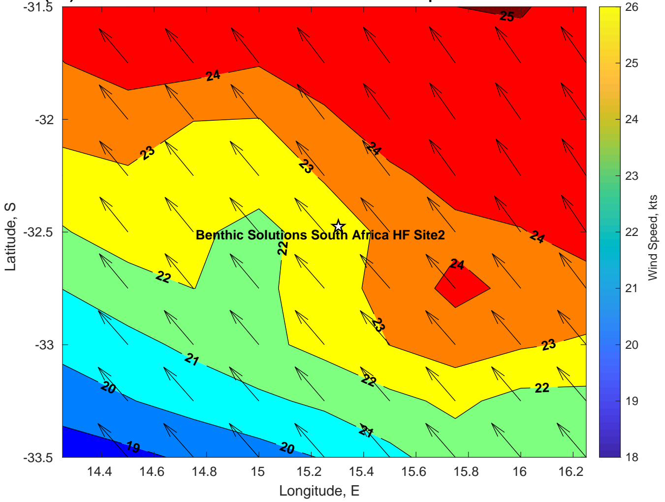
Winds (kts) for Benthic Solutions South Africa HF Site2 at 02-Apr-2025 09:00:00
